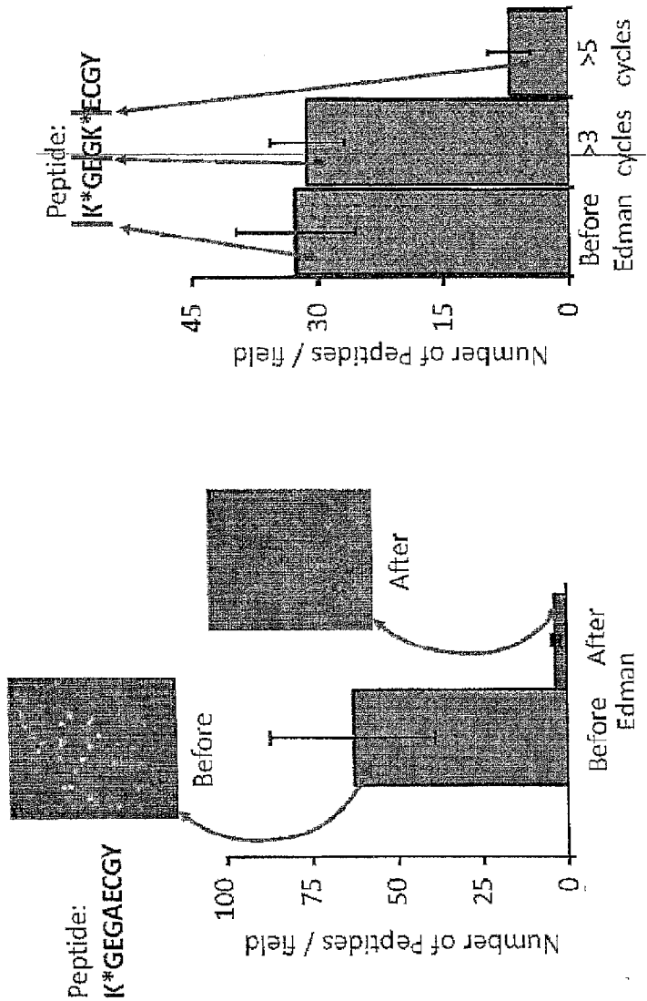
FIGURE 15 Edman degradation on single peptide molecules
