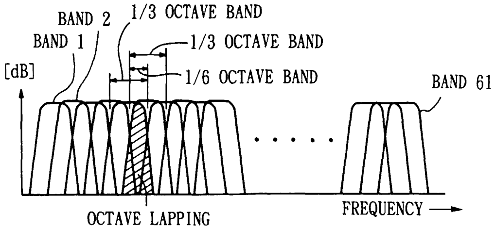
1/3 OCTAVE BAND, 1/6 OCTAVE PITCH
