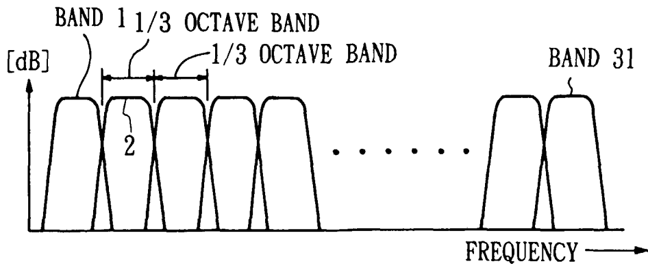
1/3 OCTAVE BAND, 1/3 OCTAVE PITCH
