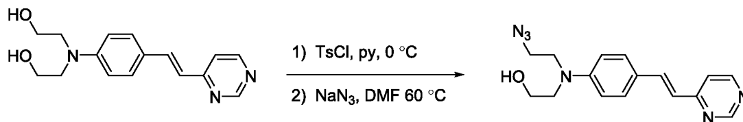
Compound iii
