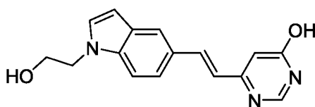
Compound xii
