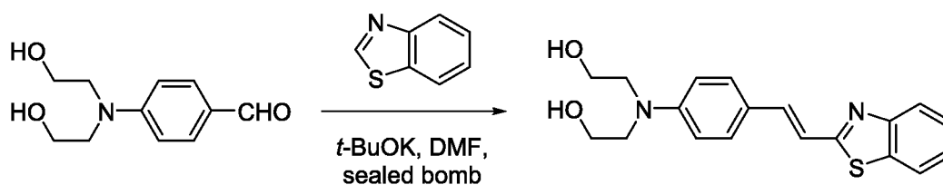
Compound iv
