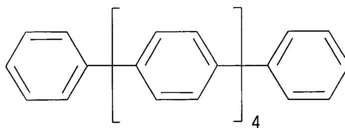
P-sexiphenyl
