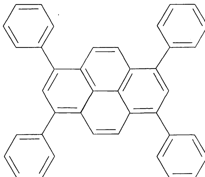
1,3,6,8-tetraphenylpyrene
