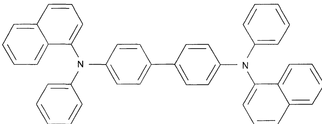
NPD
