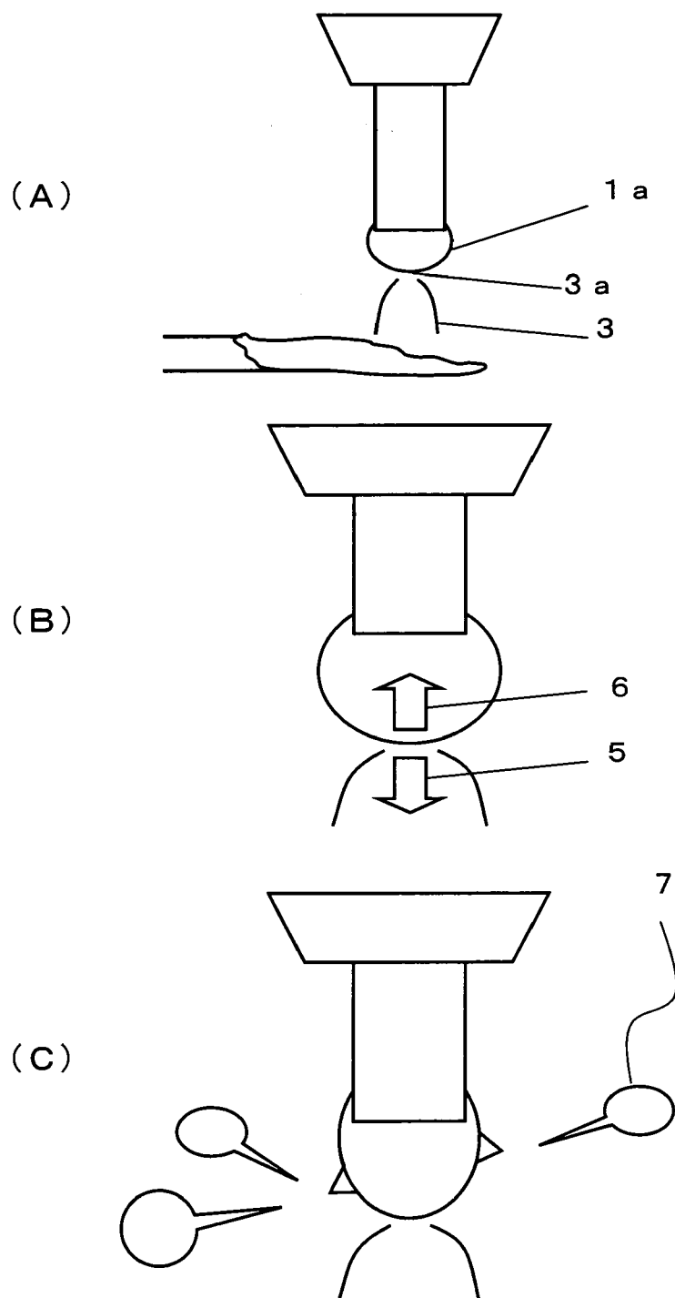
FIG. 13 PRIOR ART
