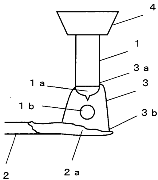
FIG. 12 PRIOR ART
