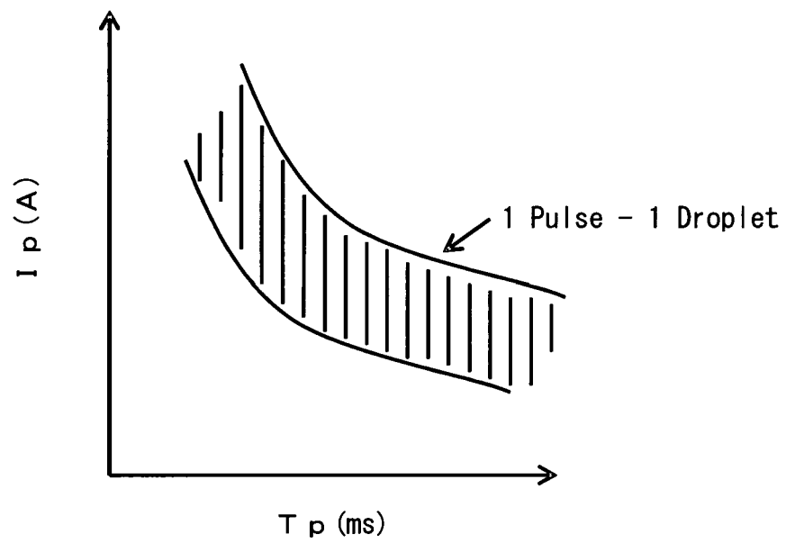
FIG. 11 PRIOR ART
