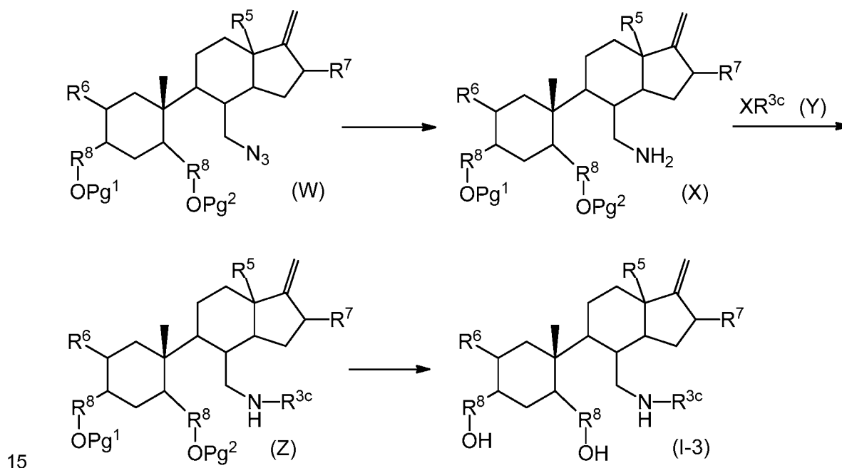
REACTION SCHEME 3
