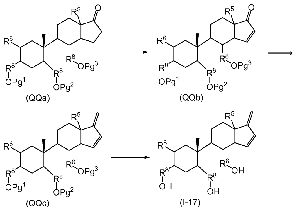
REACTION SCHEME 16
