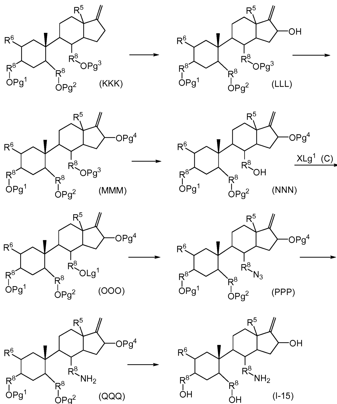
REACTION SCHEME 14
