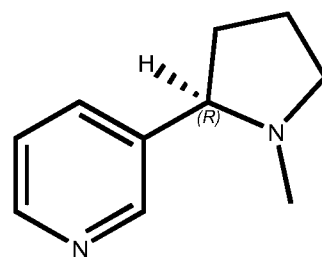
Formula I-c (R)-Nicotine
