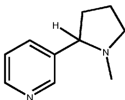
Formula I-a mixture of (R)- and (S)-Nicotine
