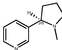
Formula I-c (R)-Nicotine
