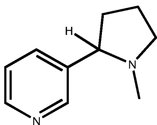
10 Formula I-a mixture of (R)- and (S)-Nicotine
