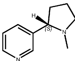
Formula I-b (S)-Nicotine
