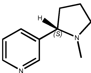
Formula I-b (S)-Nicotine
