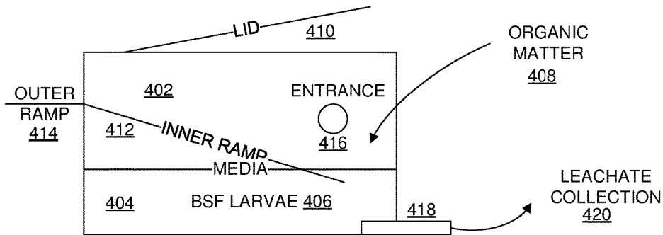
FIG. 4 BSF AUTO FISH FEEDER (BSF) 122
