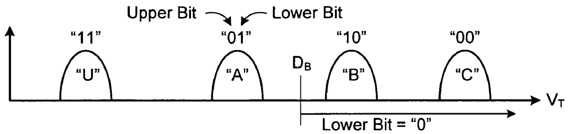
Lower Page Read (LM New Code)
