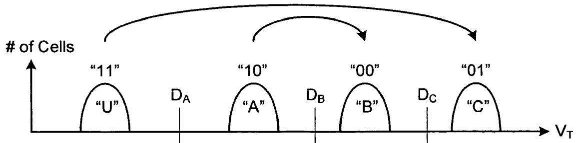
Upper Page Programming (Conventional Gray Code)
