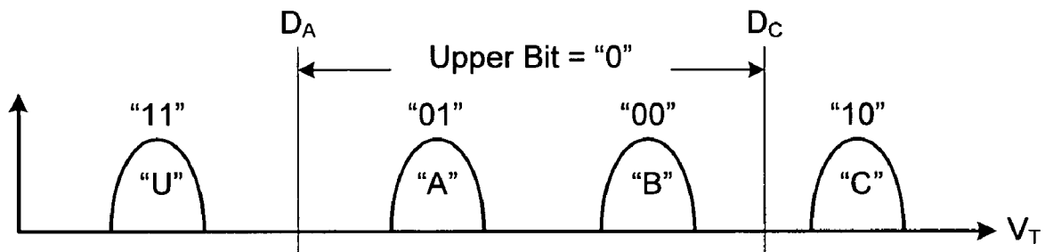
Upper Page Read (LM Gray Code)
