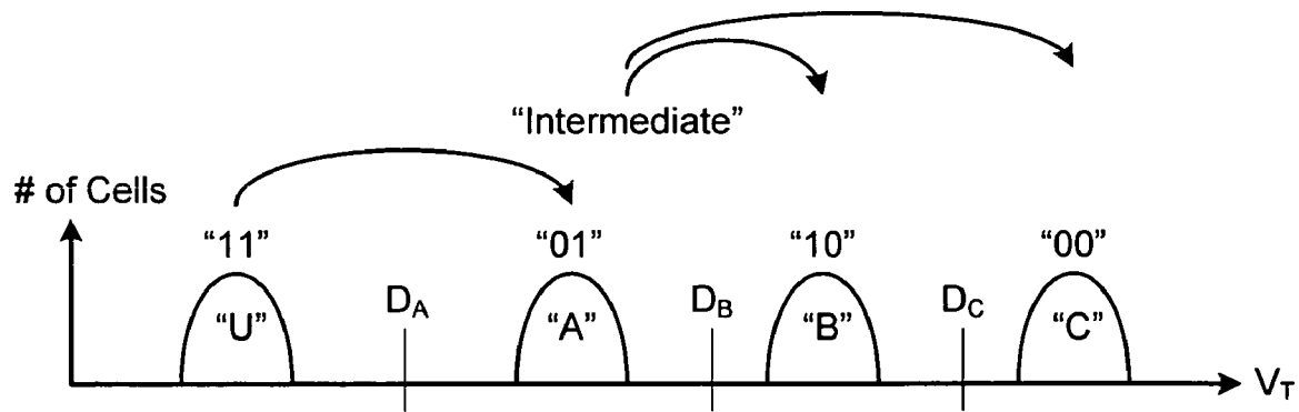
Upper Page Programming (LM New Code)
