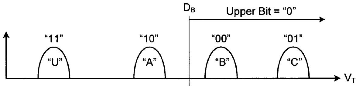
Upper Page Read (Conventional Gray Code)
