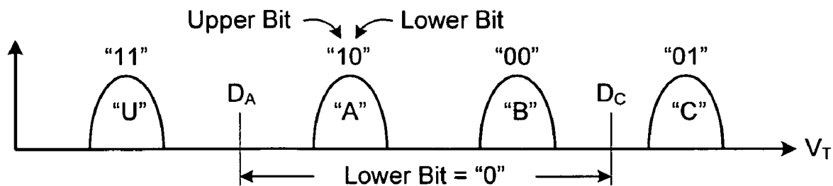
Lower Page Read (Conventional Gray Code)
