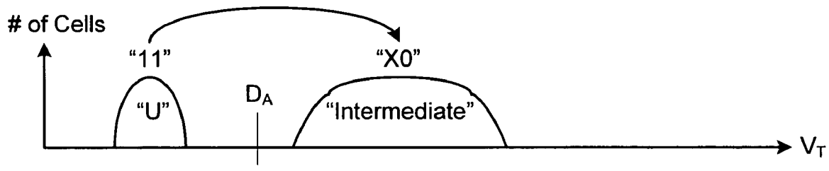
Lower Page Programming (LM New Code)
