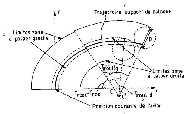
FIG. 2B 1 BOUNDARIES OF LEFT ZONE TO BE TRACED 2 TRACING SUPPORT TRAJECTORY 3 BOUNDARIES OF RIGHT ZONE TO BE TRACED 4 CURRENT AIRCRAFT POSITION 5 ROLL
