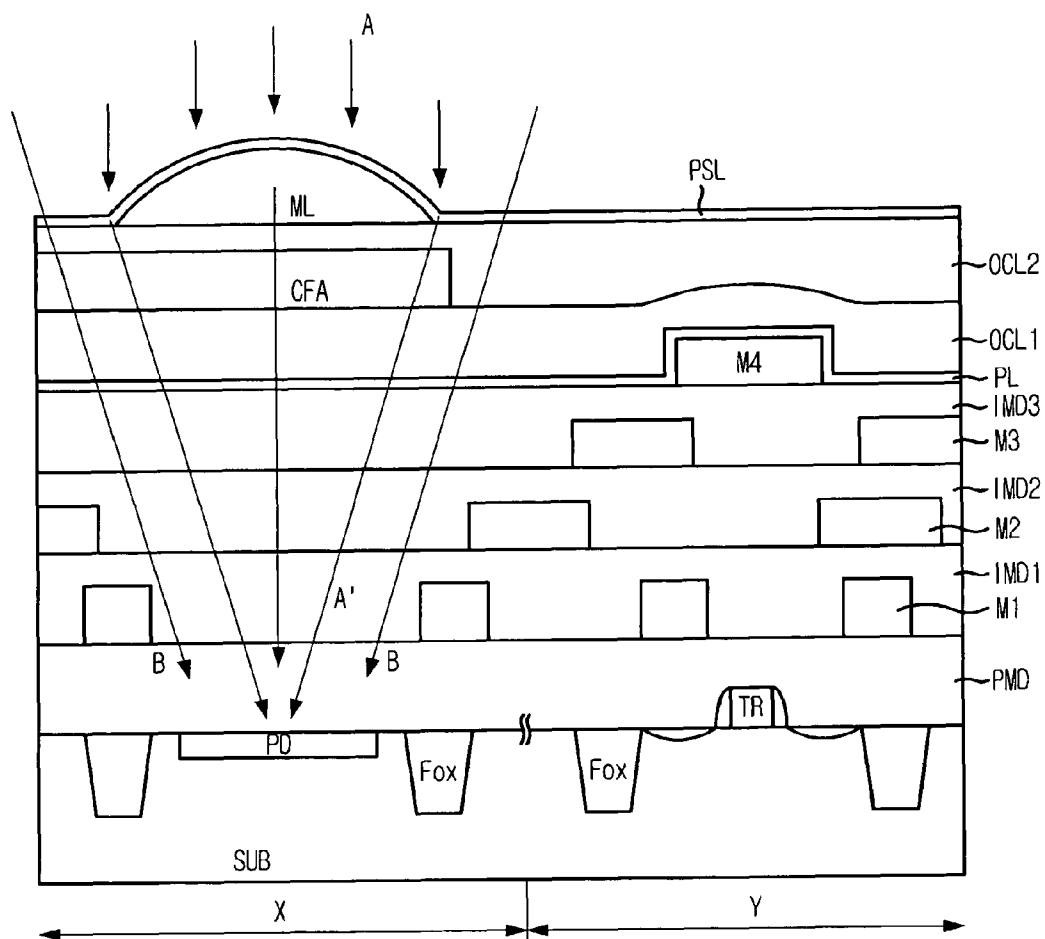
FIG. 2 (RELATED ART)
