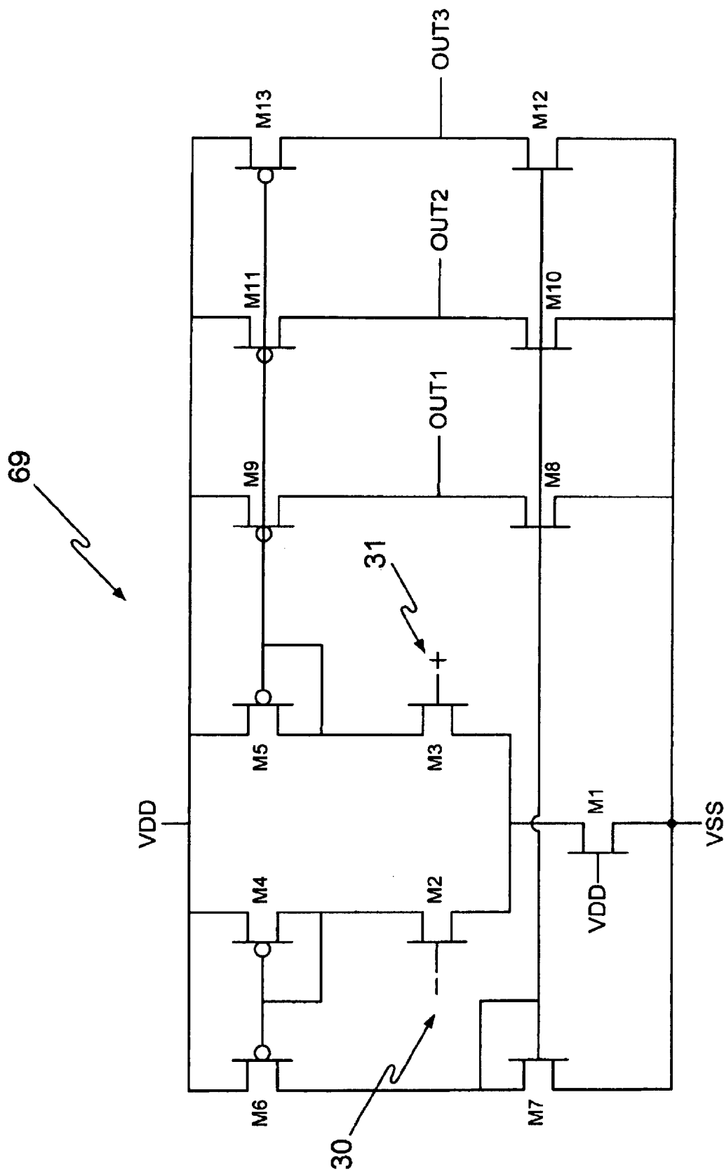
Fig. 5: Multi-output Differential-to-single-ended Amplifier
