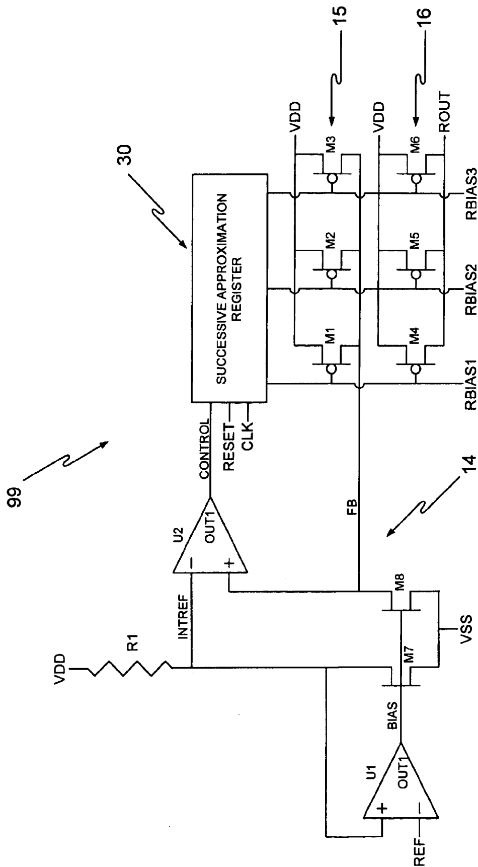
Fig. 1: Prior-Art Resistor Mirror
