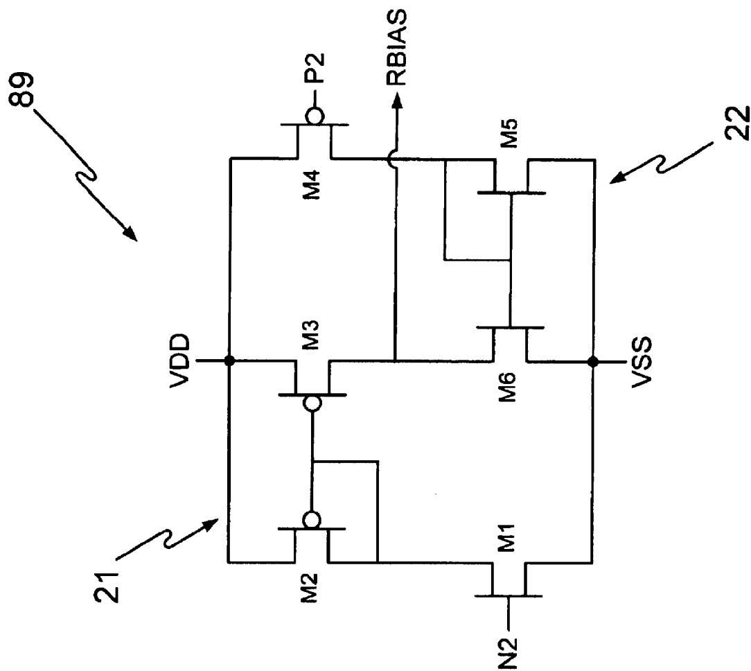
Fig. 6: Offset Control Circuit
