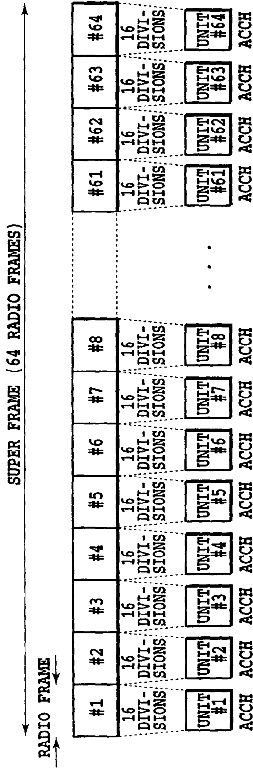
MAPPING INTO 256ksps DEDICATED PHYSICAL CHANNEL
