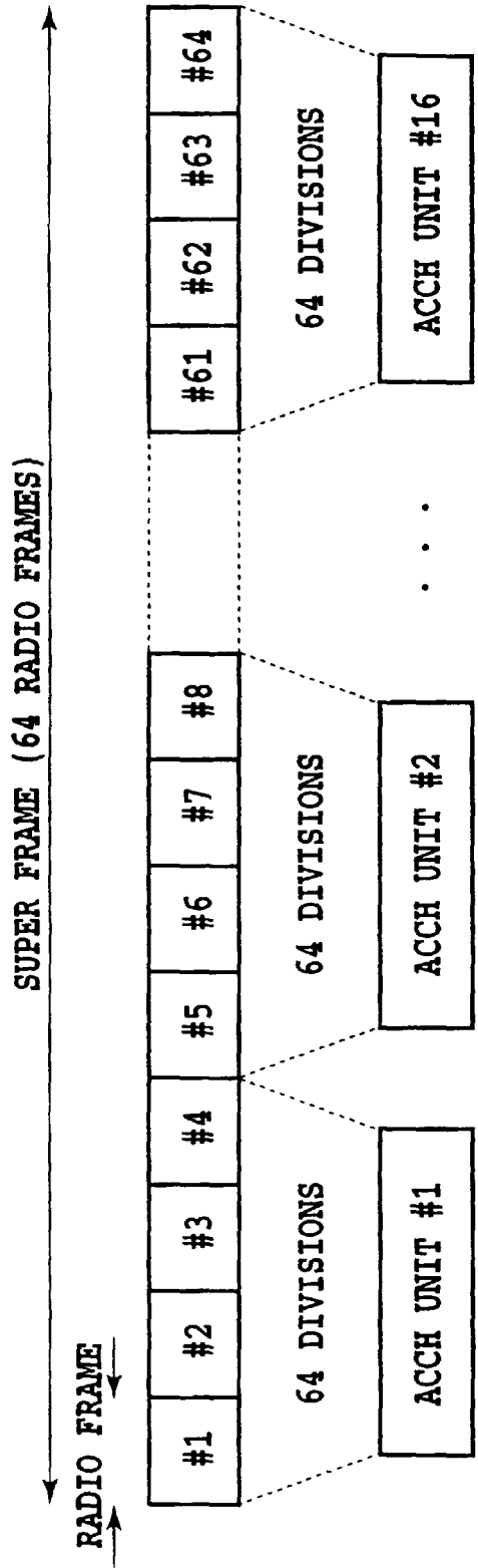
MAPPING INTO 32 OR 64ksp DEDICATED PHYSICAL CHANNEL
