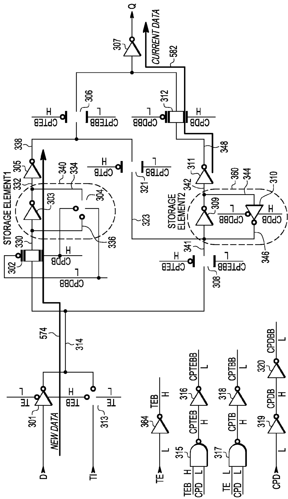
NORMAL MODE CLOCK LOW OPERATION
