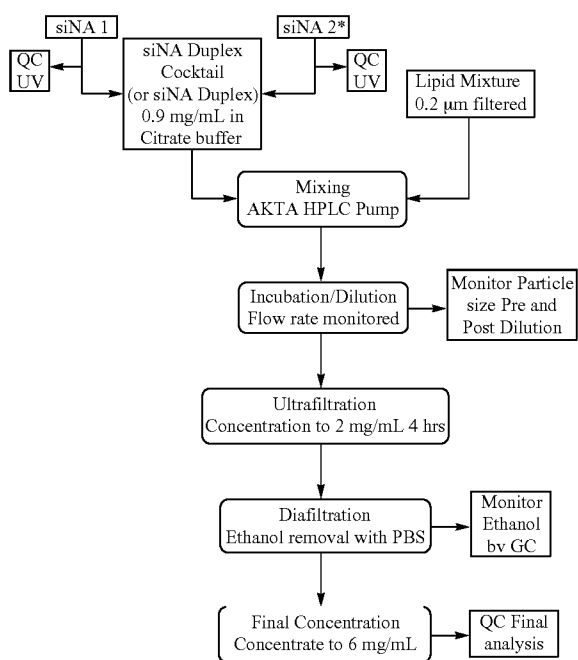
LNP PROCESS FLOW CHART
