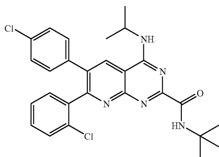
N-(Tert-butyl)-7-(2-chlorophenyl)-6-(4-chlorophenyl)-4-(isopropylamino)pyrido[2,3-d]pyrimidine-2-carboxamide
