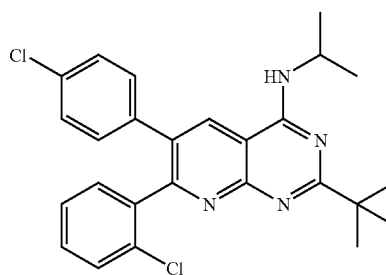
2-Tert-butyl-7-(2-chlorophenyl)-6-(4-chlorophenyl)-N-isopropylpyrido[2,3-d]pyrimidin-4-amine
