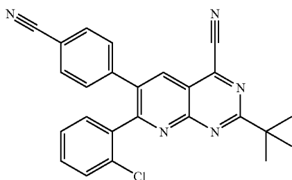
2-Tert-butyl-7-(2-chlorophenyl)-6-(4-cyanophenyl) pyrido[2,3-d]pyrimidine-4-carbonitrile
