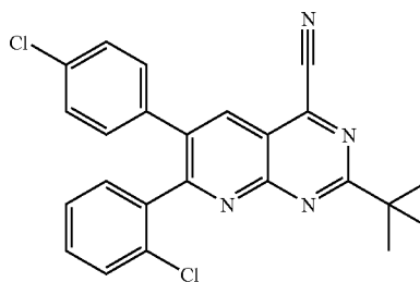
2-Tert-butyl-7-(2-chlorophenyl)-6-(4-chlorophenyl) pyrido[2,3-d]pyrimidine-4-carbonitrile
