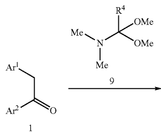
Scheme 3
