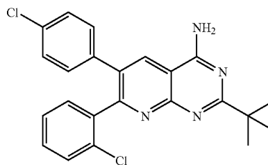
2-Tert-butyl-7-(2-chlorophenyl)-6-(4-chlorophenyl) pyrido[2,3-d]pyrimidin-4-amine
