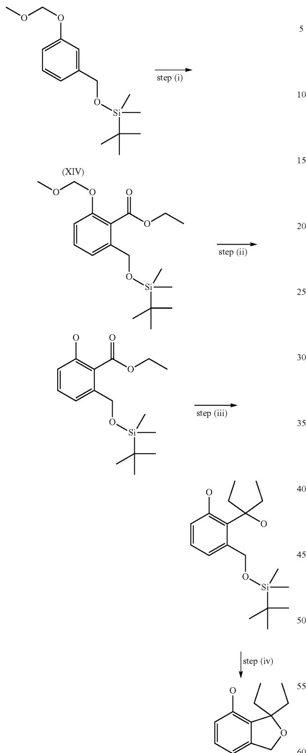
Scheme 19b
