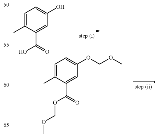
Scheme 9b
