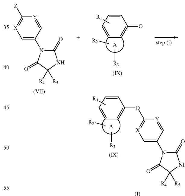
Scheme 1b
