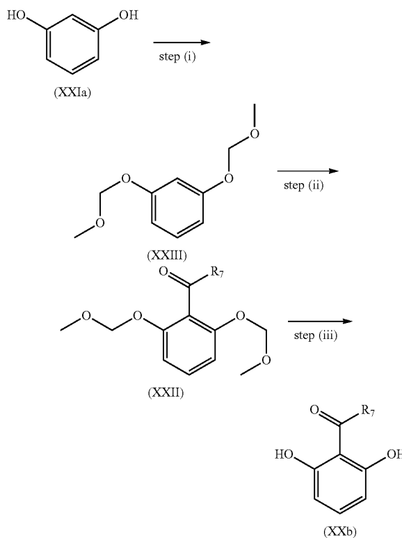
Scheme 12
