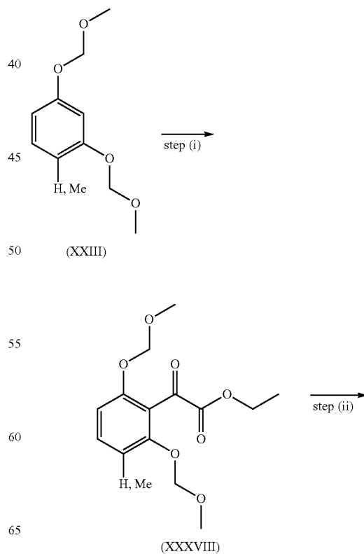
Scheme 16
