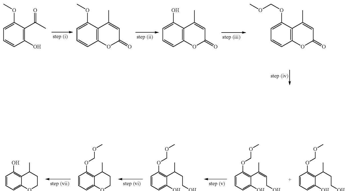
Scheme 17b
