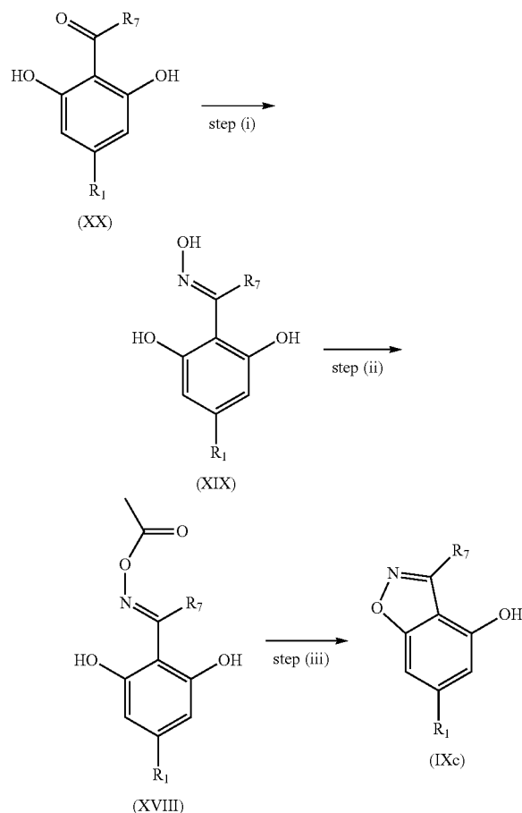
Scheme 10
