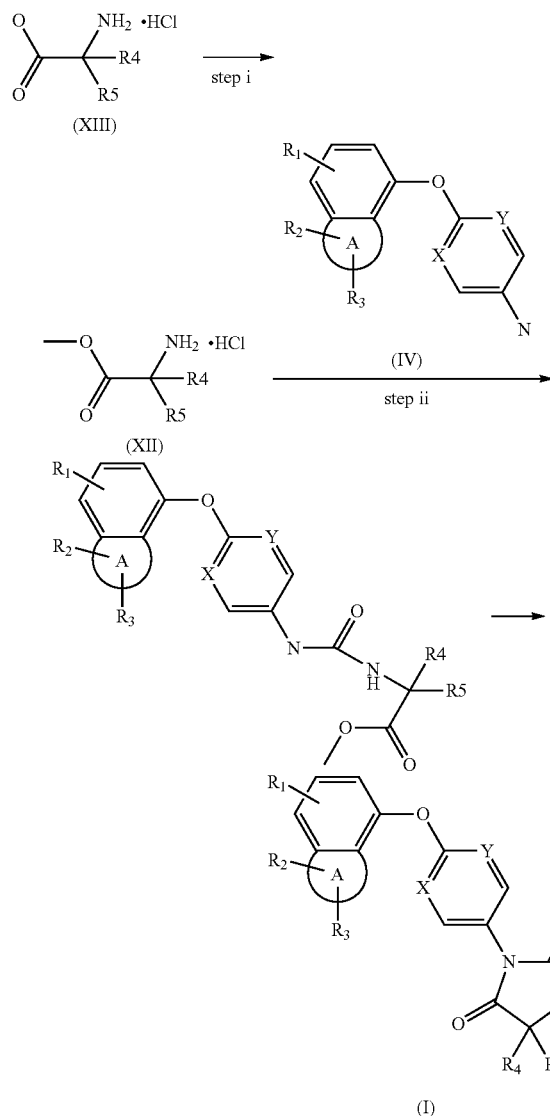
Scheme 1c
