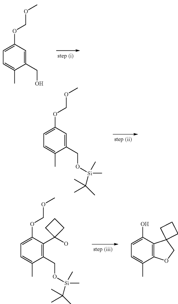
Scheme 8b
