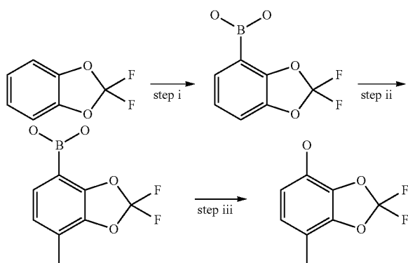
Scheme 22
