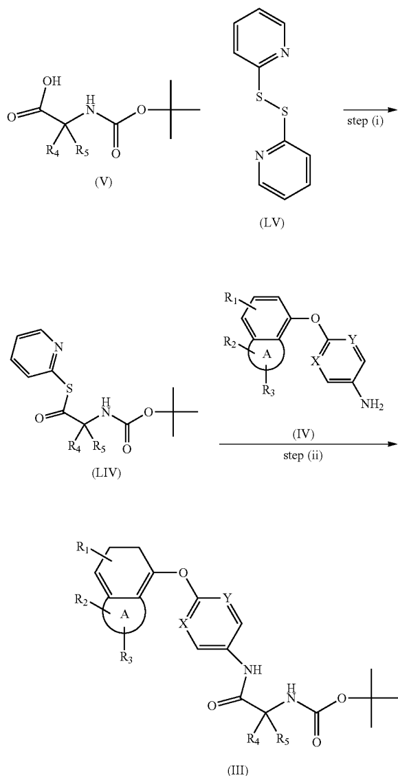
Scheme 25
