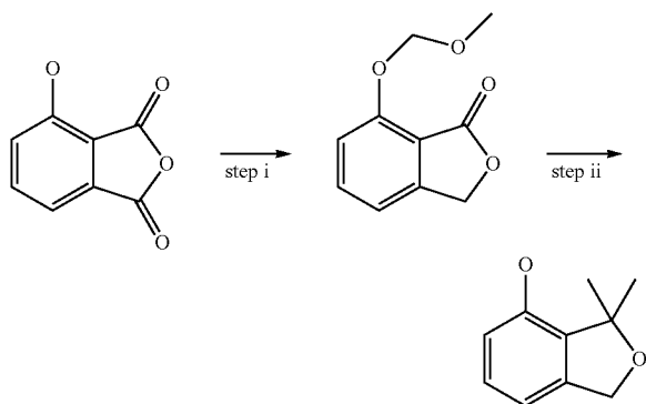
Scheme 21
