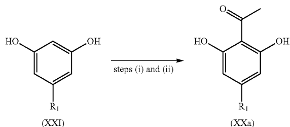
Scheme 11
