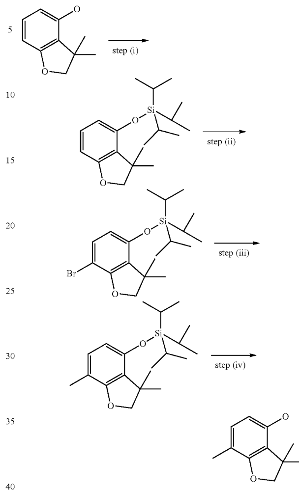
Scheme 13b
