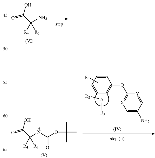
Scheme 2b
