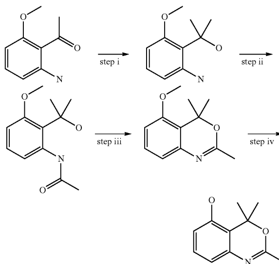
Scheme 24
