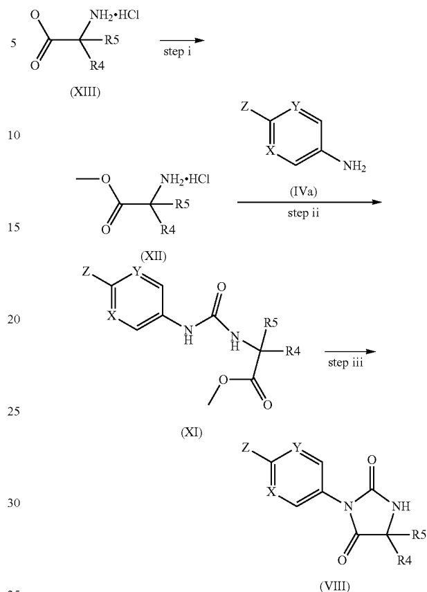
Scheme 26
