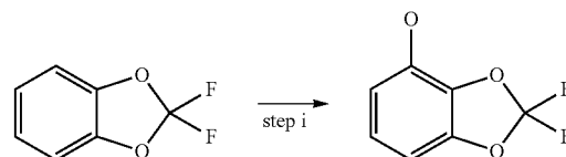
Scheme 23
