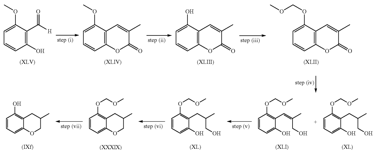
Scheme 17a
