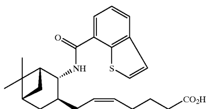
Reference compound 2
