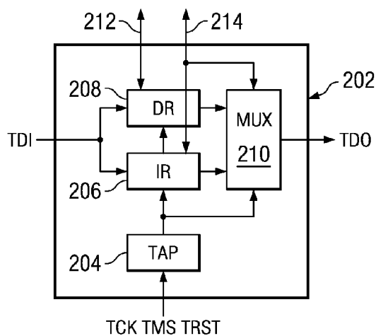
FIG. 2 (PRIOR ART)
