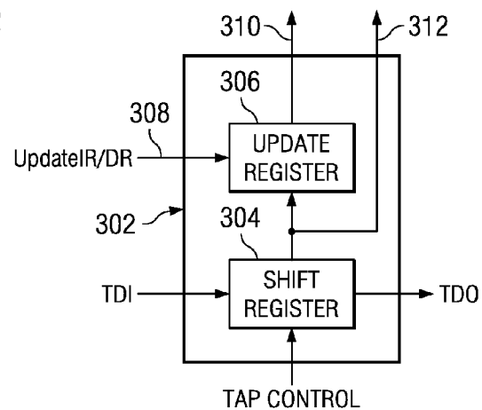
FIG. 3 (PRIOR ART)
