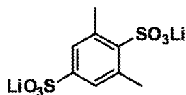
lithium 2,6-dimethylbenzene-1,4-disulfonate
