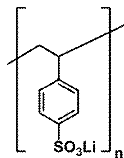
Poly(lithium-4-styrenesulfonate)
