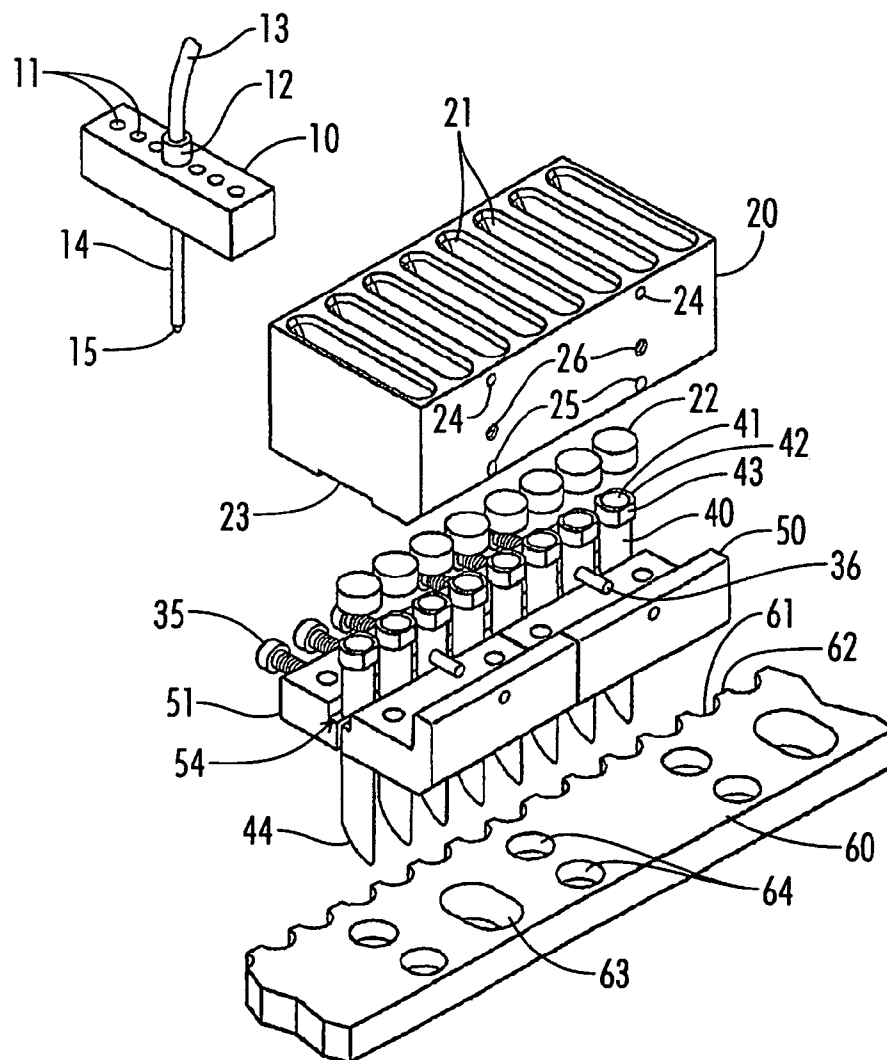
FIG. 1 (PRIOR ART)
