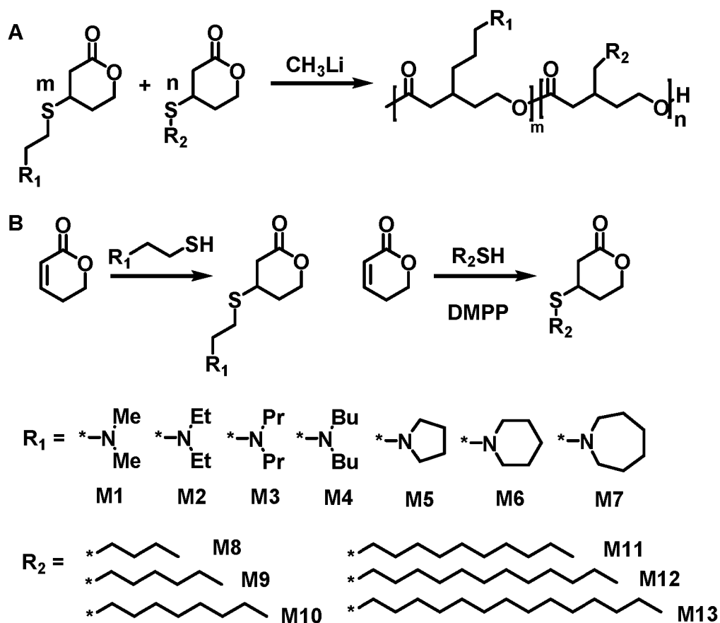
Scheme 3: Polymeric Synthesis
