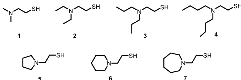
Scheme 1: Synthesis of thiol containing amines
