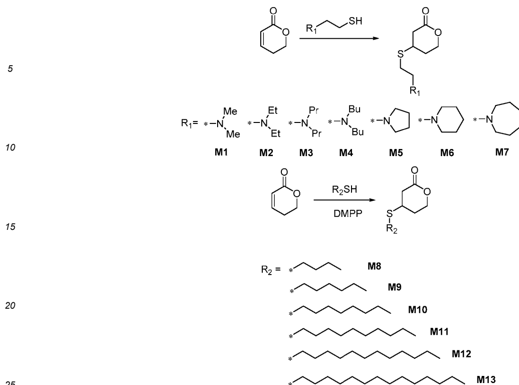
Scheme 2. Synthesis of monomers M1-M13
