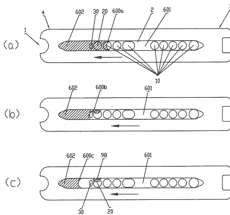
Fig. 6 (PRIOR ART)
