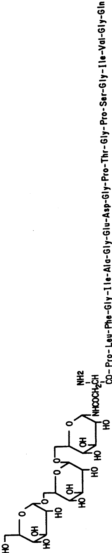
STRUCTURE OF NEPHRITOGENOSIDE
