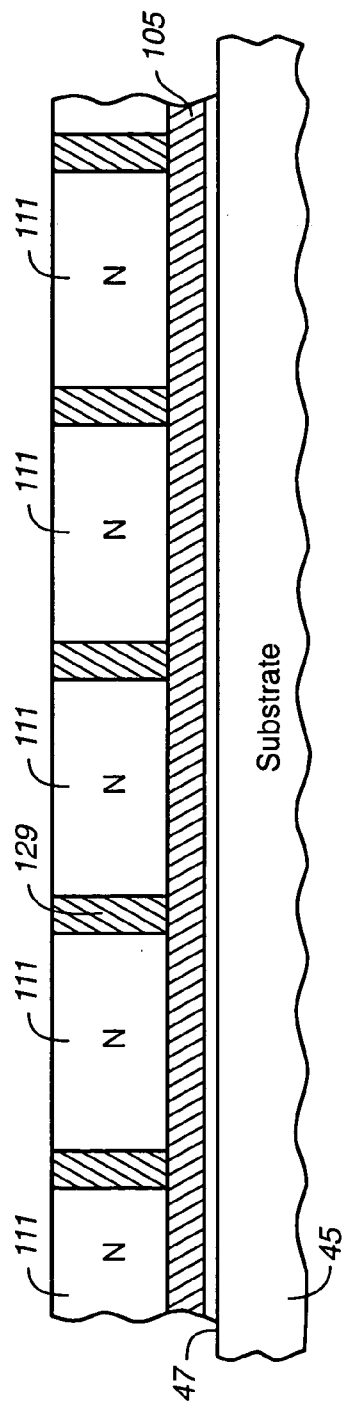
FIG. 5 (Section I-I)
