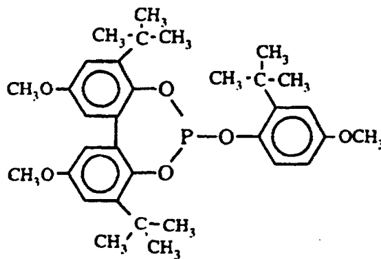
Ligand A
