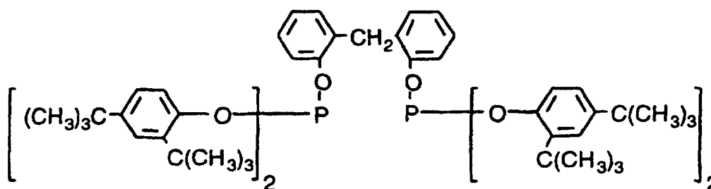
Ligand U
