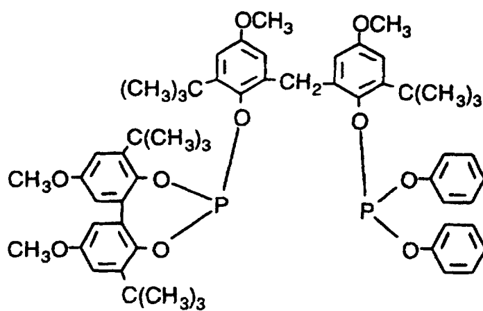
Ligand R
