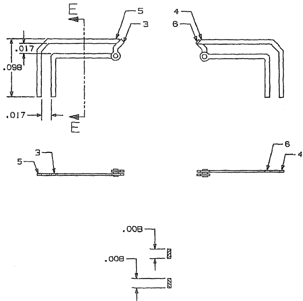
SECTION E-E
