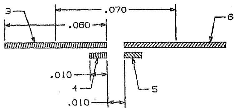
SECTION F-F
