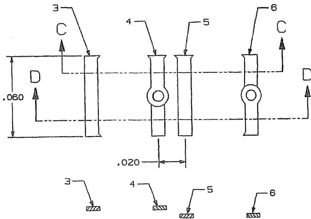
SECTION C-C
