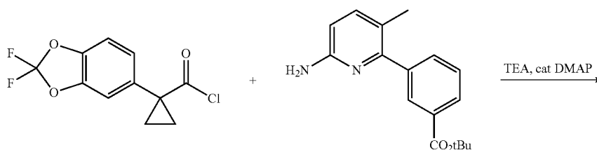
Scheme 4. Formation of an acid salt of 3-(6-(1-(2,2-difluorobenzo[d][1,3]dioxol-5-yl)cyclopropanecarboxamido)-3-methylpyridin-2-yl)benzoic acid.
