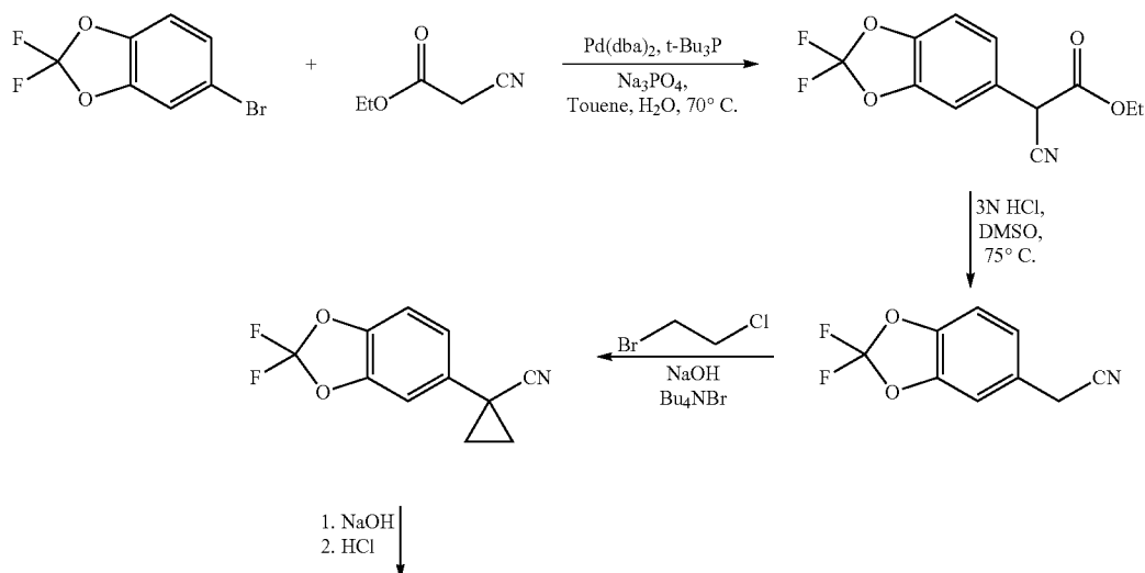
Scheme 2. Alternative synthesis of the acid chloride moiety.
