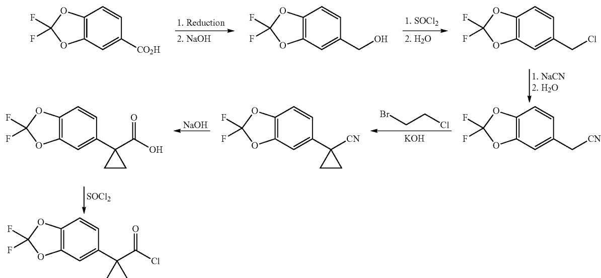
Scheme 1. Synthesis of the acid chloride moiety.
