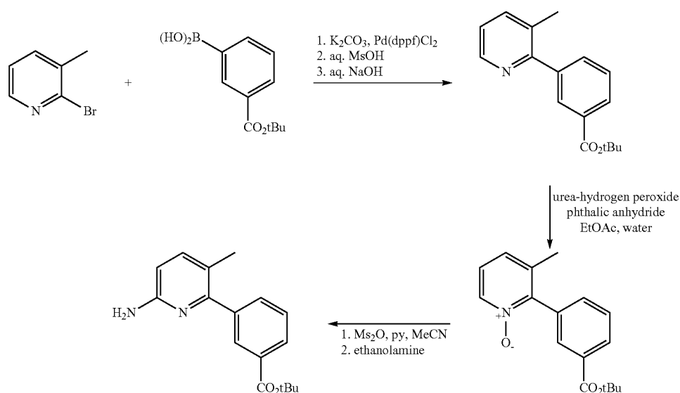
Scheme 3. Synthesis of the amine moiety.
