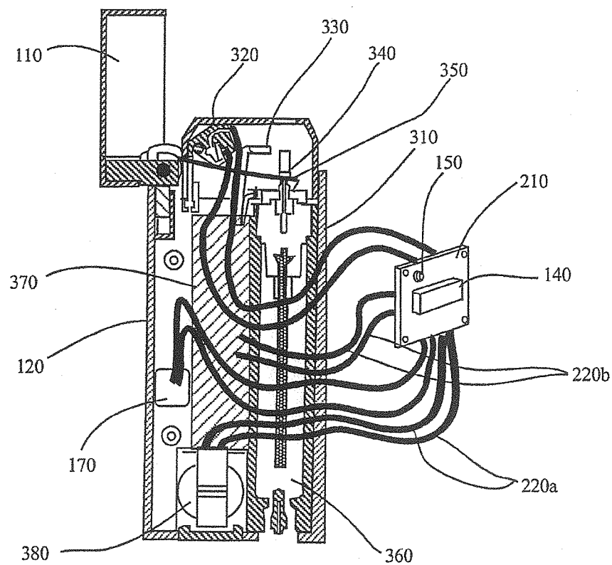
Portable Biometric Lighter Cross-Sectional View
