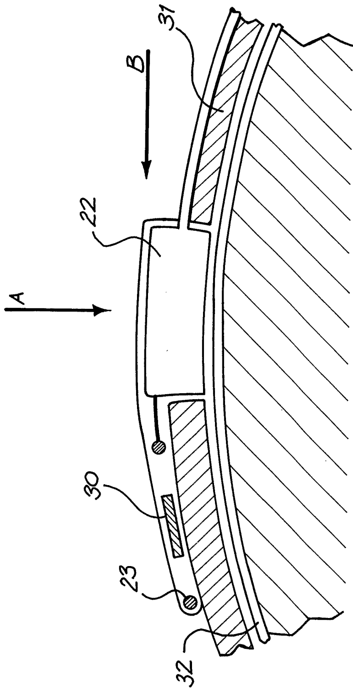
FIG. 2 (PRIOR ART)
