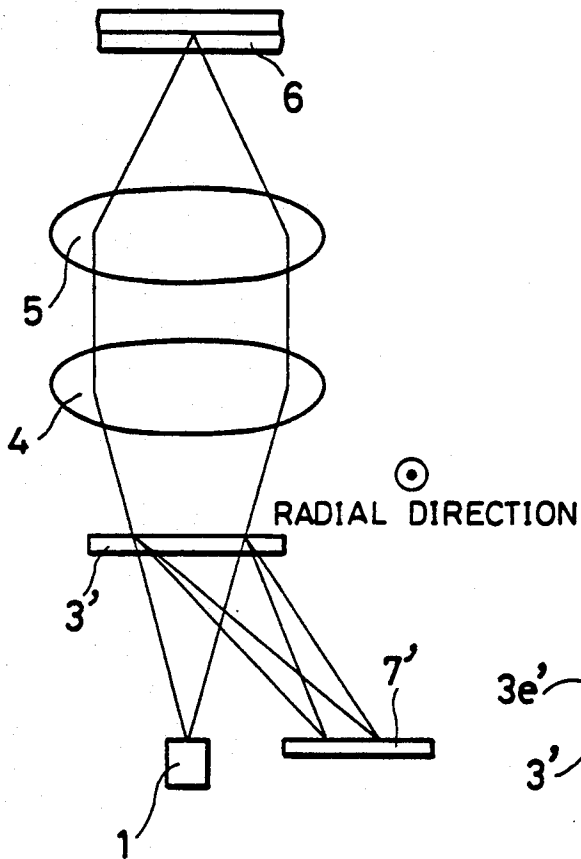
FIG. 12 PRIOR ART RADIAL DIRECTION
