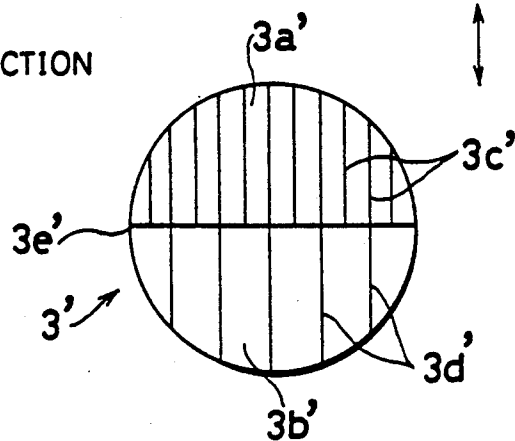
FIG. 12 PRIOR ART RADIAL DIRECTION
