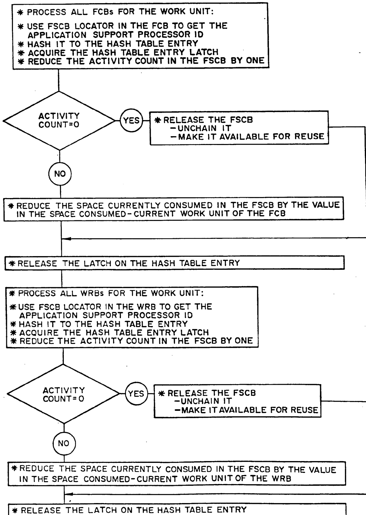
FIG.9 ROLLBACK OPERATION
