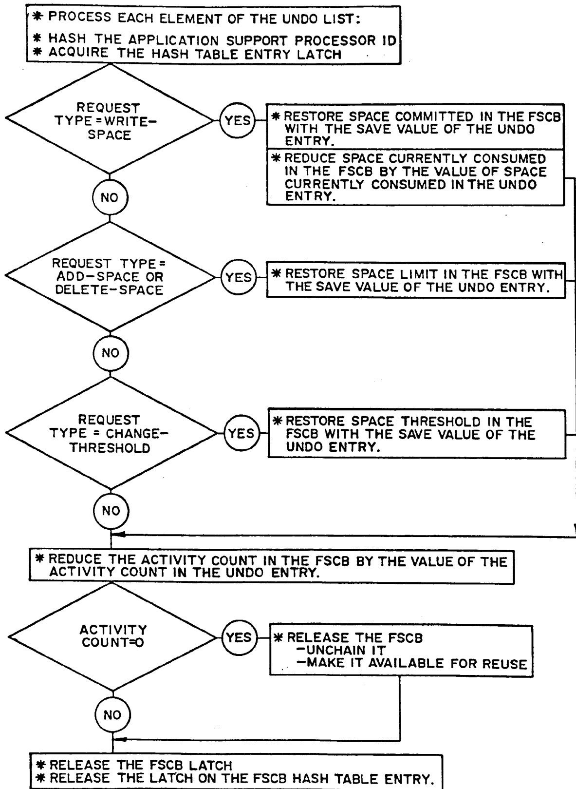
FIG.10 UNDO OPERATION
