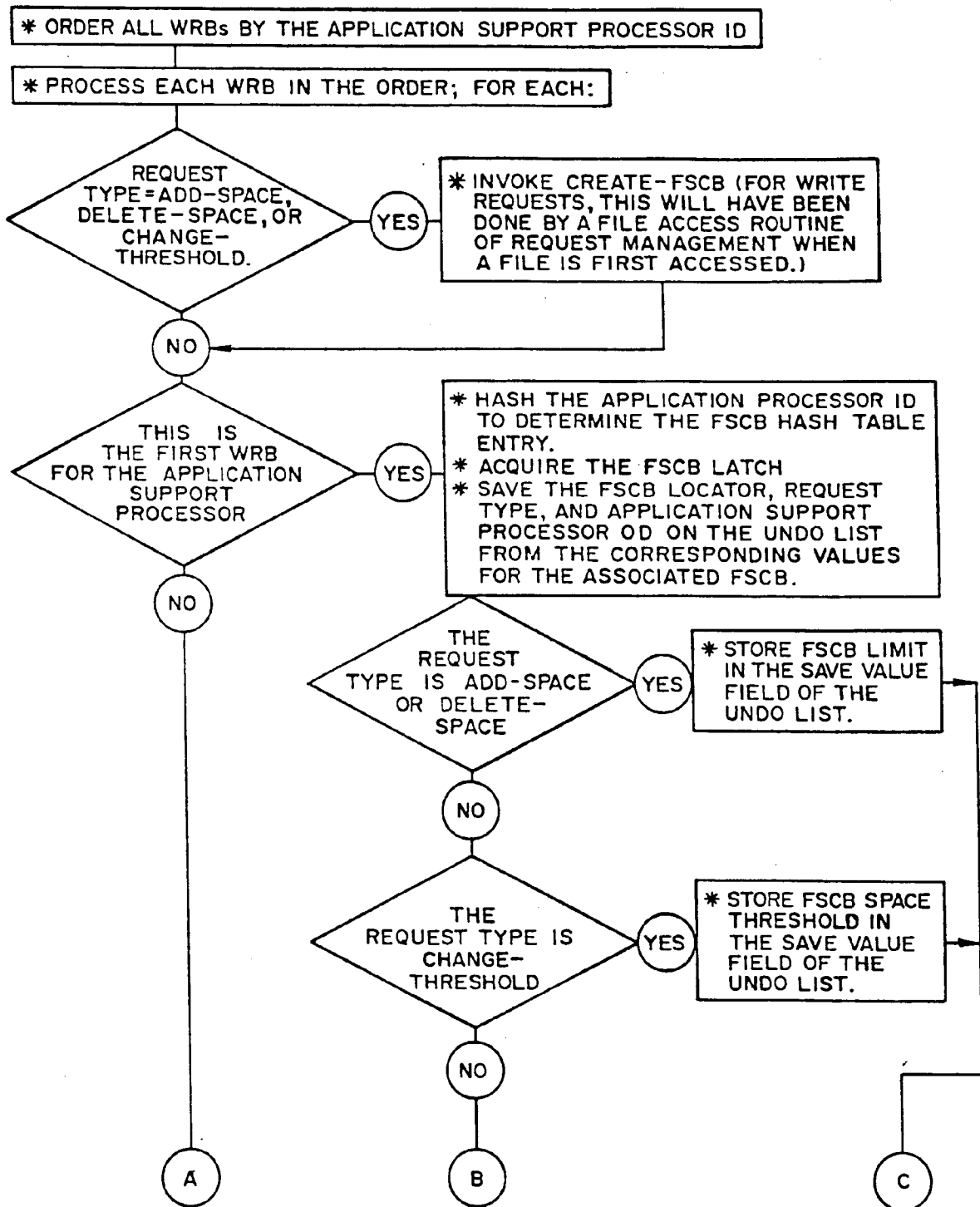
FIG.6 COMMIT OPERATION
