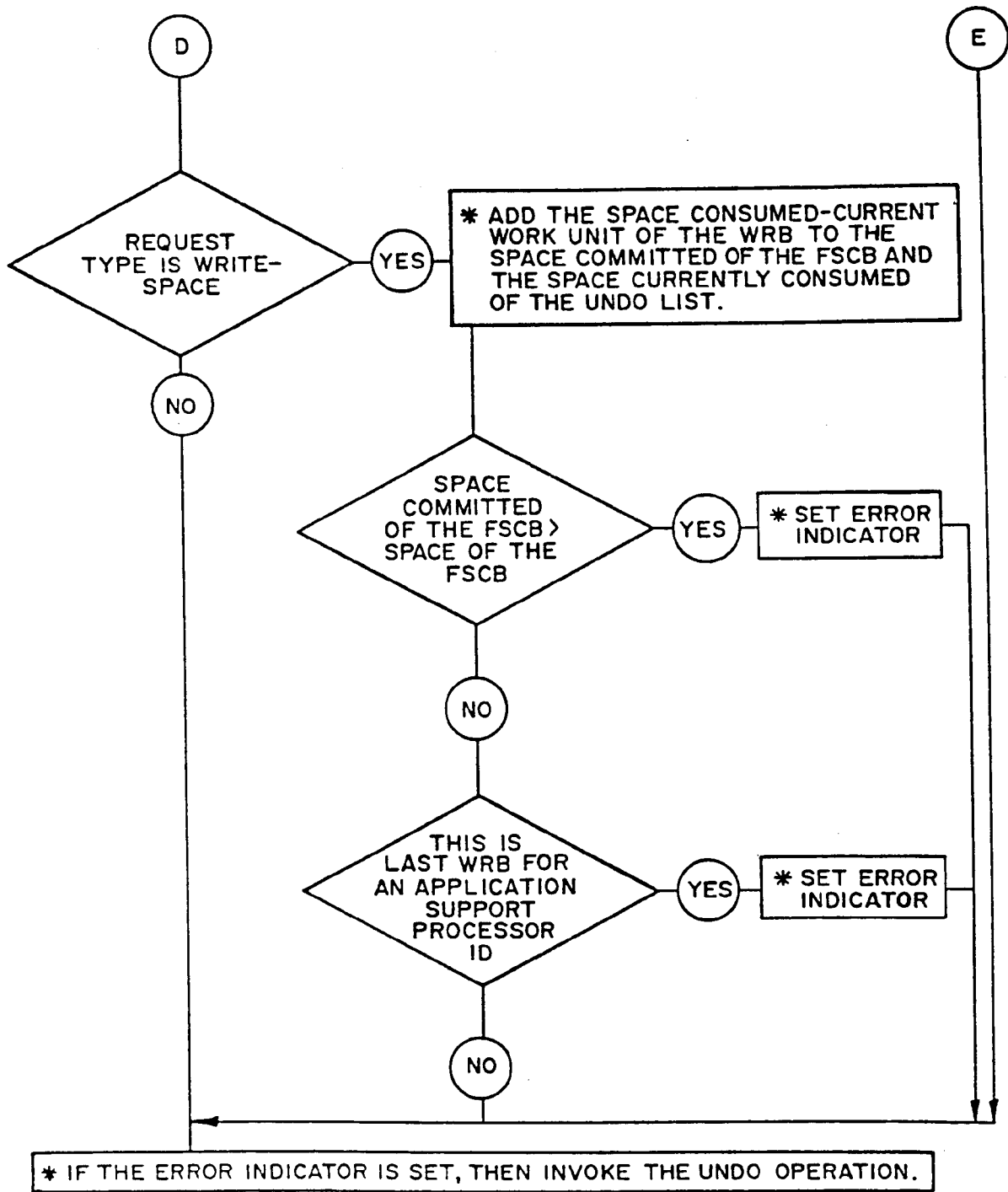
FIG.8 COMMIT OPERATION
