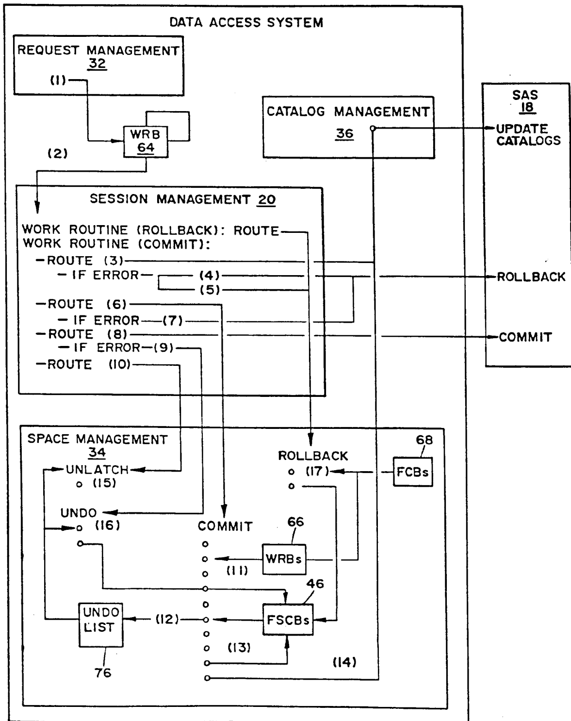
FIG.5 SPACE MANAGEMENT END OF WORK UNIT PROCESSING
