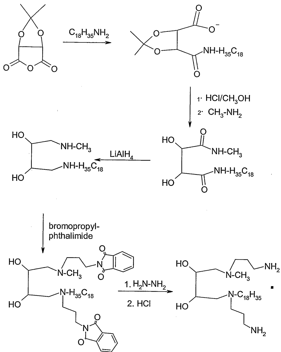
Scheme 1 : Generalized synthesis of cationic glycolipid analogs
