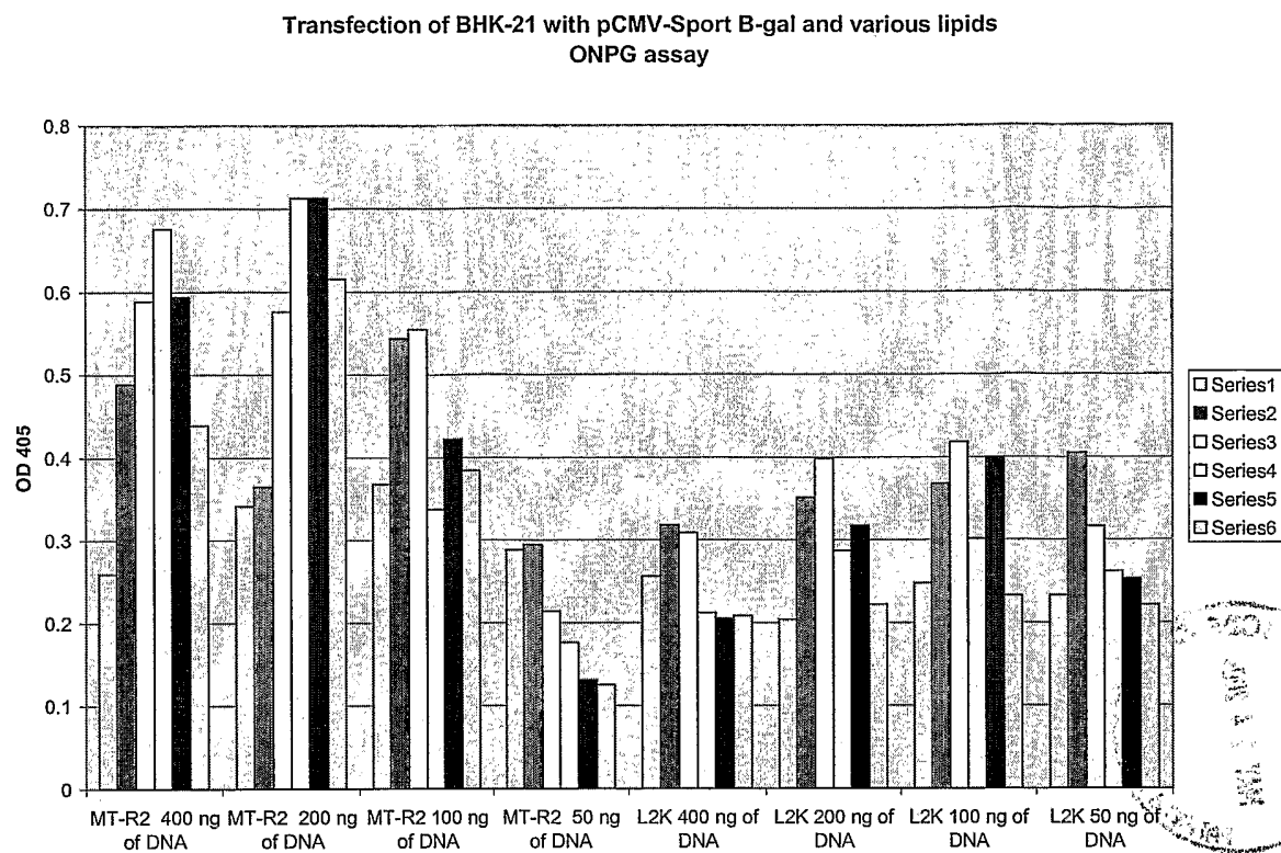
FIGURE 3: Transfection of BHK-21 with pMCMV-Sport \beta -gal MT-R2 and lipofectamine 2000
