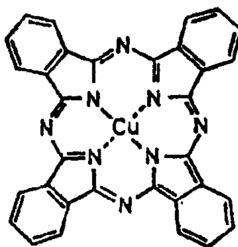
Cu-Phthalocyanine
