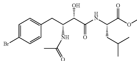
mono-acyl ubenimex bromide
