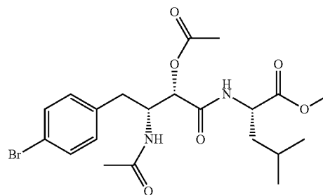
di-acyl ubenimex bromide
