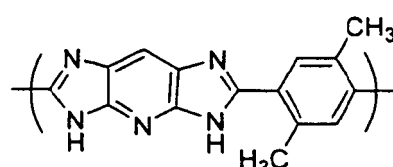
Chemical Formula 6-8
