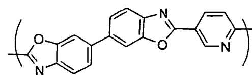
Chemical Formula 8-3
