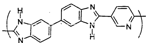
Chemical Formula 8-1
