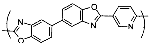
Chemical Formula 8-7
