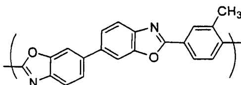
Chemical Formula 9-3
