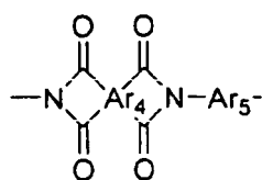
(Chemical Formula 12)
