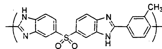
Chemical Formula 9-2
