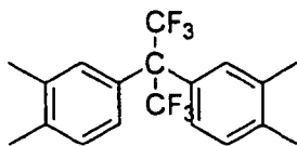
Chemical Formula 13-6
