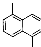
Chemical Formula 3-15
