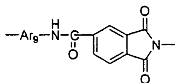
(Chemical Formula 20)
