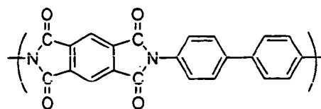
Chemical Formula 15-2
