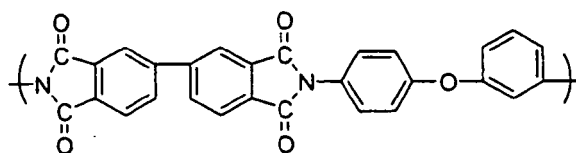
Chemical Formula 15-7
