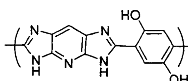
Chemical Formula 10-6
