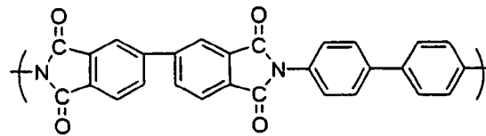
Chemical Formula 15-8
