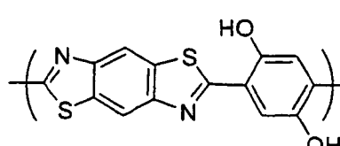
Chemical Formula 10-4
