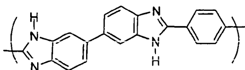
Chemical Formula 7-1
