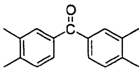
Chemical Formula 13-5
