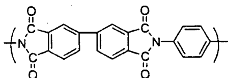
Chemical Formula 15-5
