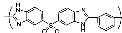
Chemical Formula 7-8
