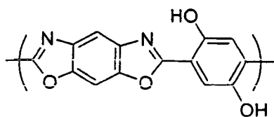
Chemical Formula 10-1
