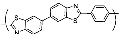
Chemical Formula 7-5
