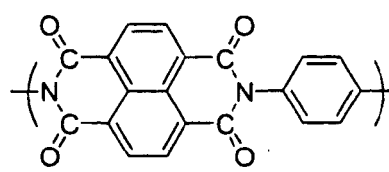
Chemical Formula 16-4
