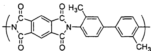
Chemical Formula 16-3
