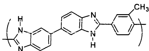
Chemical Formula 9-1
