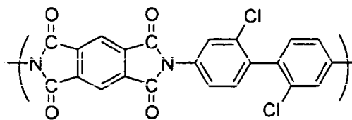
Chemical Formula 16-2
