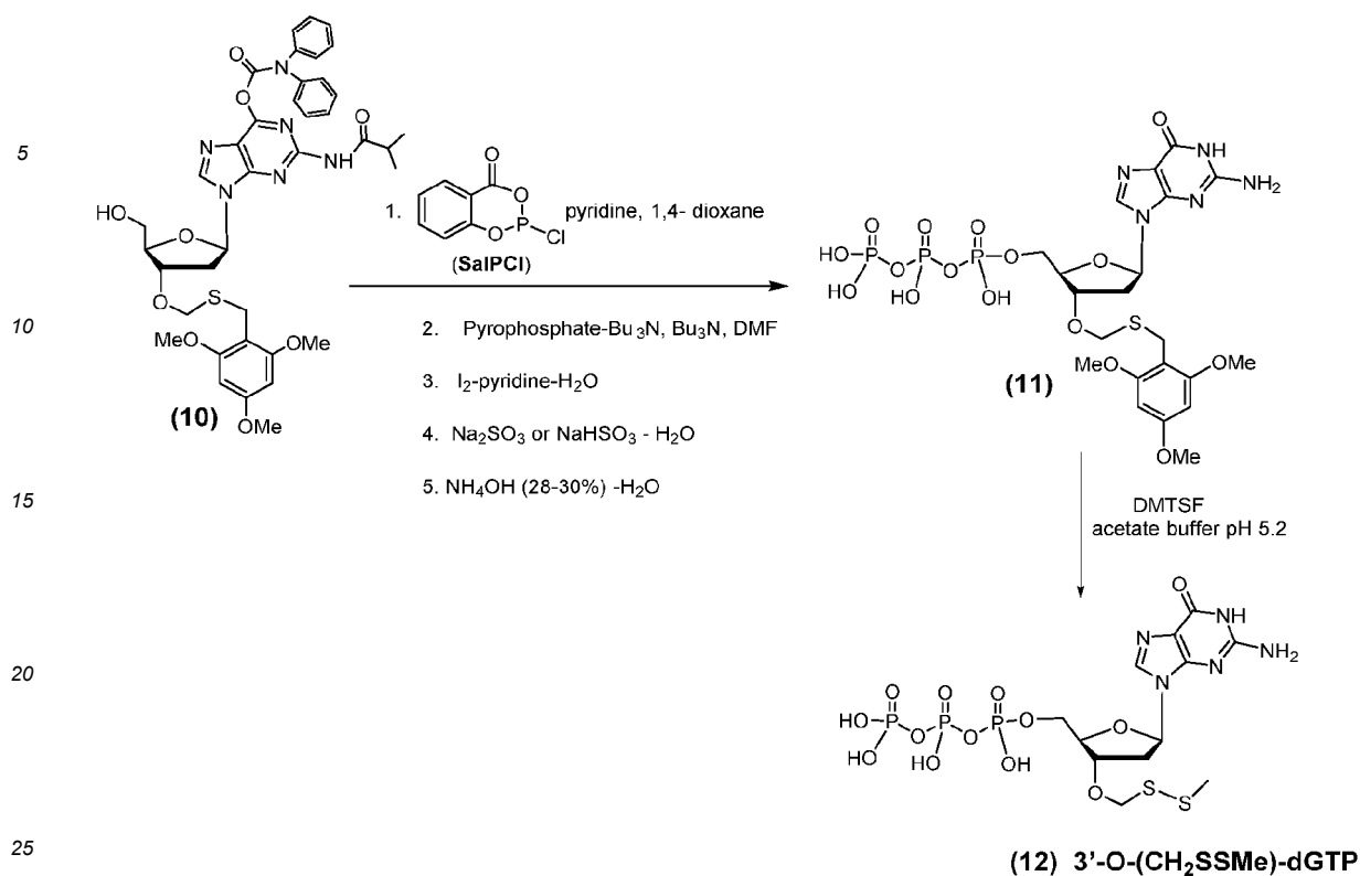
Scheme 4: Triphosphate synthesis by Eckstein triphosphate synthesis method followed by in-situ 3'-O-CH 2 SSMe capping group installation.
