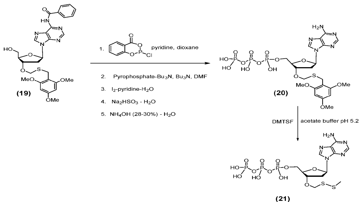
Scheme 7: Triphosphate synthesis by Eckstein method and in-situ 3'-O-CH 2 SSMe
