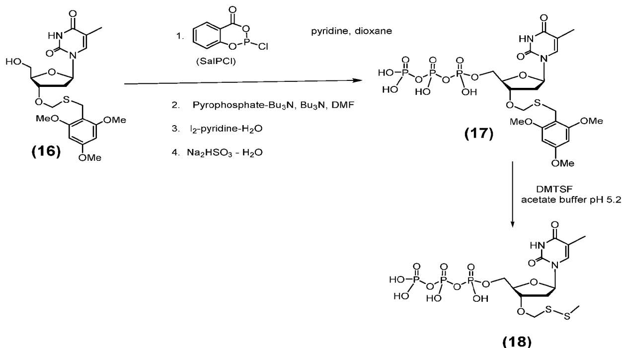
Scheme 6: Triphosphate synthesis by Eckstein method and in-situ 3'-O-CH 2 SSMe - capping group installation of dark T
