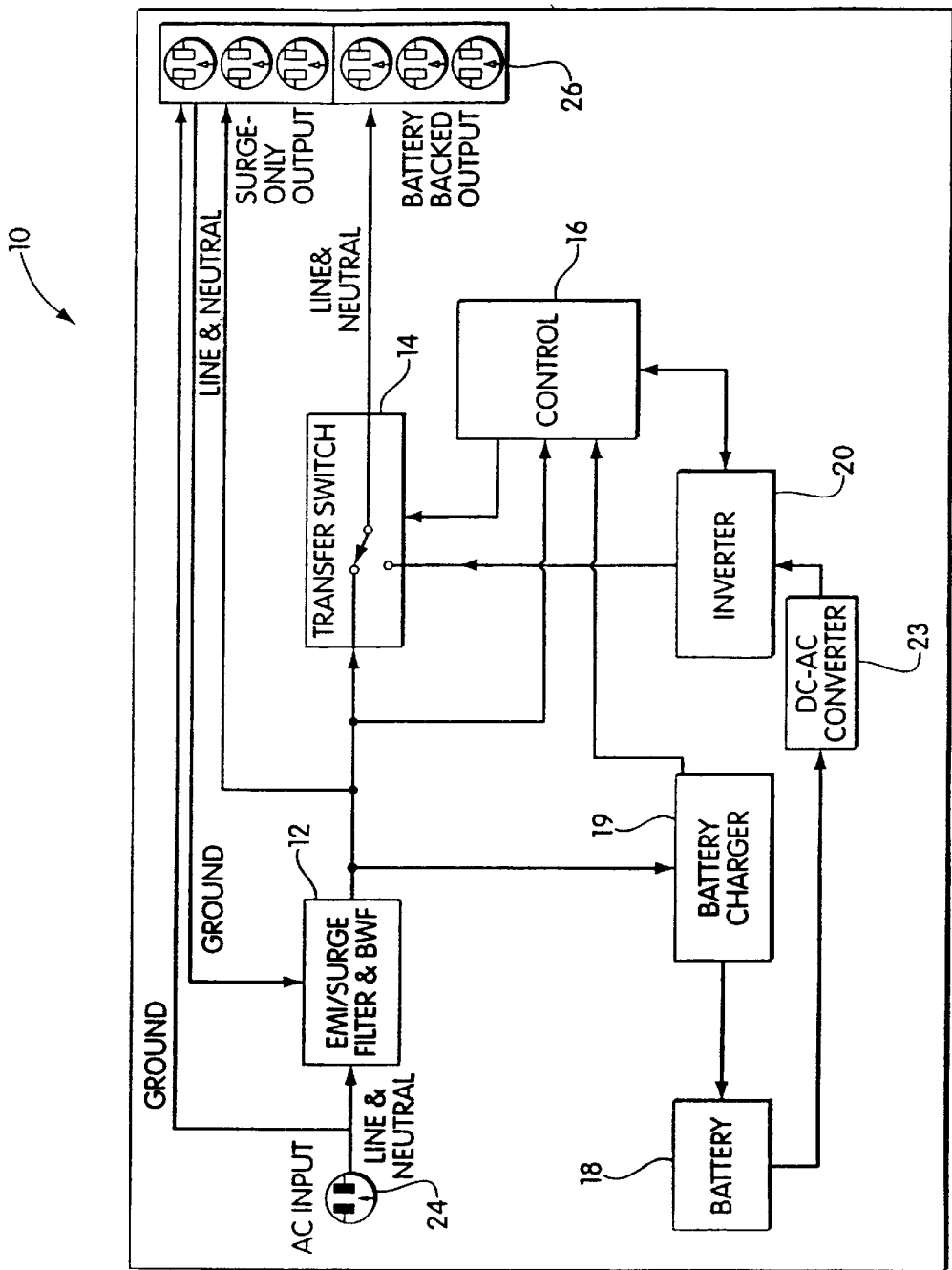
Fig. 1 (PRIOR ART)
