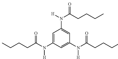
aromatic trisamide
