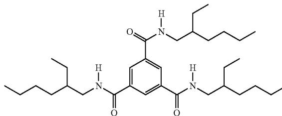
aromatic trisamide
