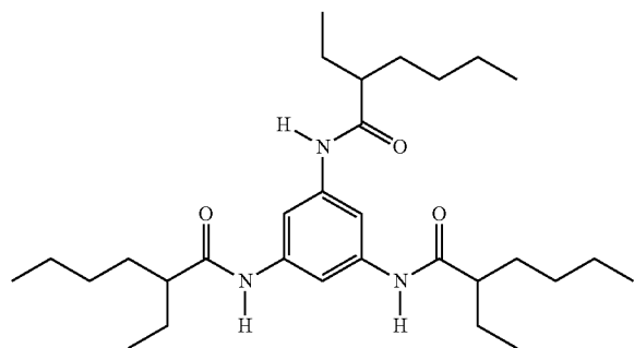
aromatic trisamide
