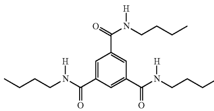
aromatic trisamide
