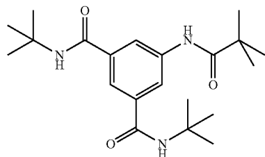
aromatic trisamide
