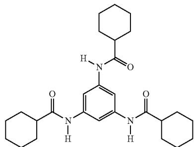
aromatic trisamide
