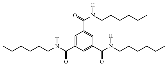
aromatic trisamide
