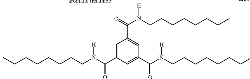
aromatic trisamide
