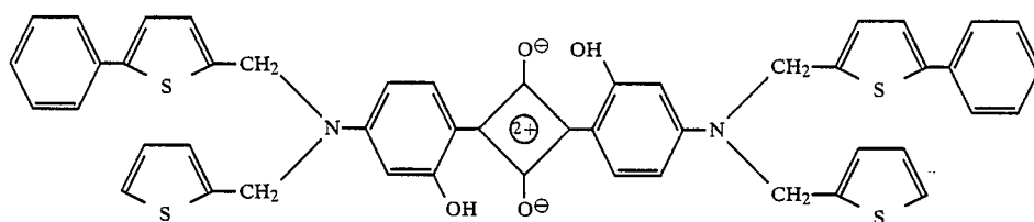
Compound No. I-31
