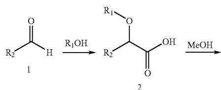
Reaction Scheme 1
