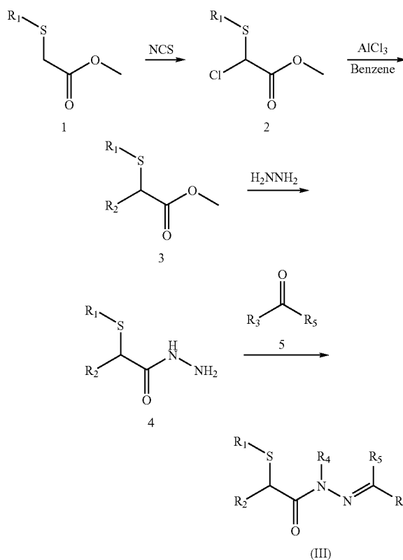
Reaction Scheme 2
