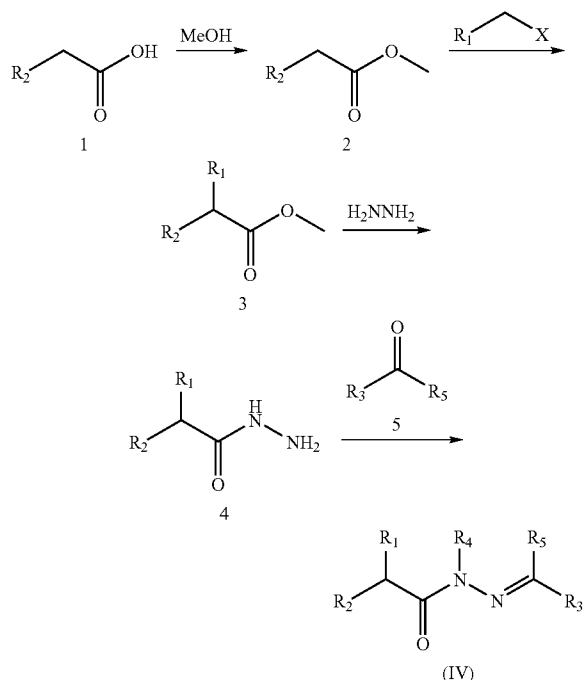
Reaction Scheme 3
