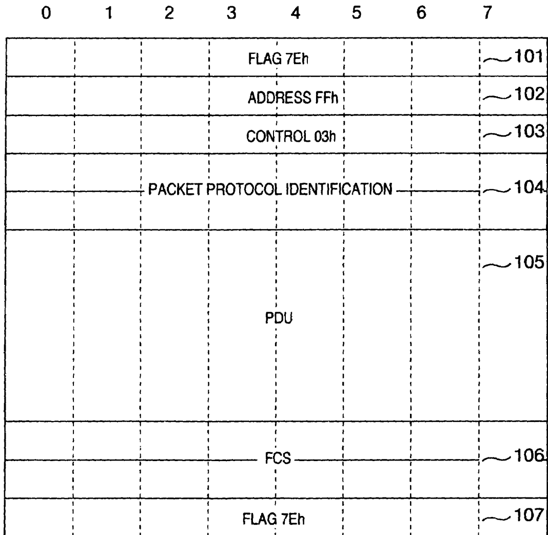
PPP FRAME FORMAT (RFC1662)
