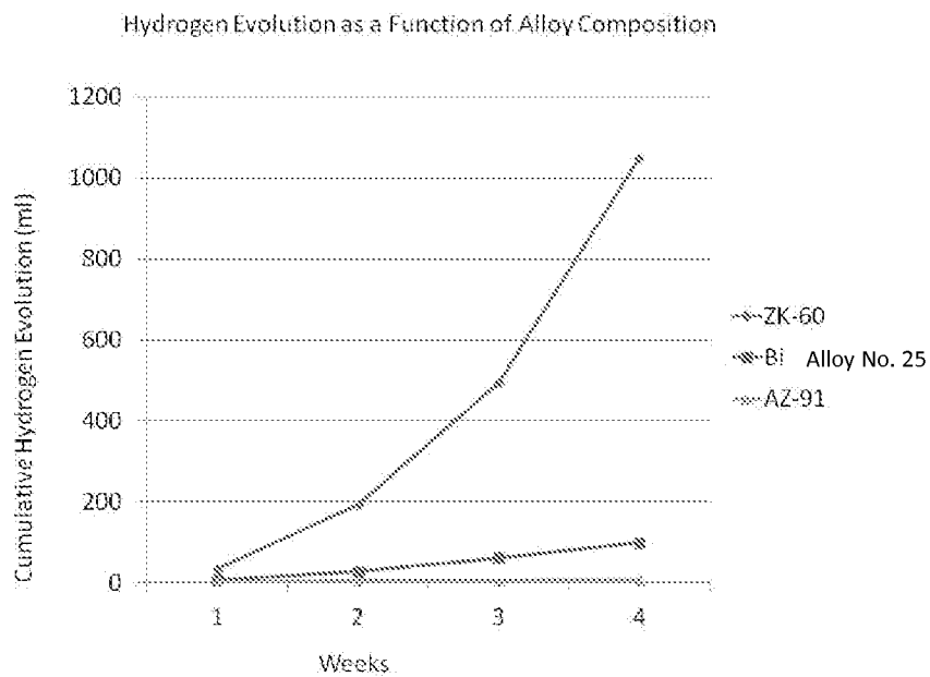
FIG. 6 - Comparison of corrosion rate of micro-alloyed Alloy No. 25 with commercially available ZK60 and AZ91D
