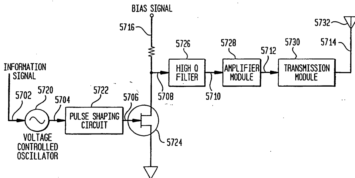
FIG. 57A TRANSMITTER IN THE FM EMBODIMENT
