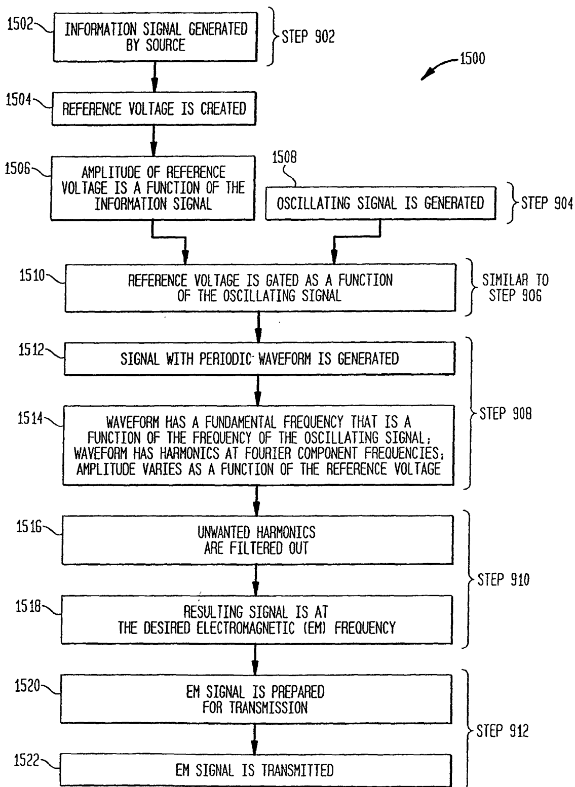
FIG. 15 AMPLITUDE MODULATION MODE
