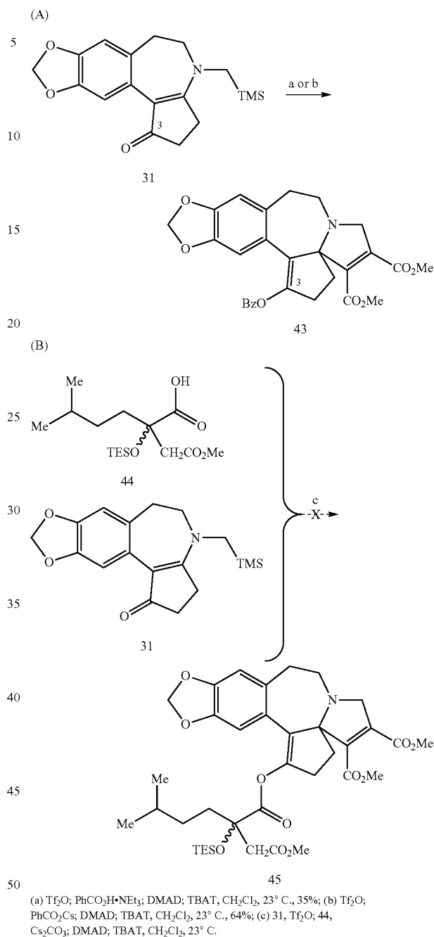
Scheme 6-1.
