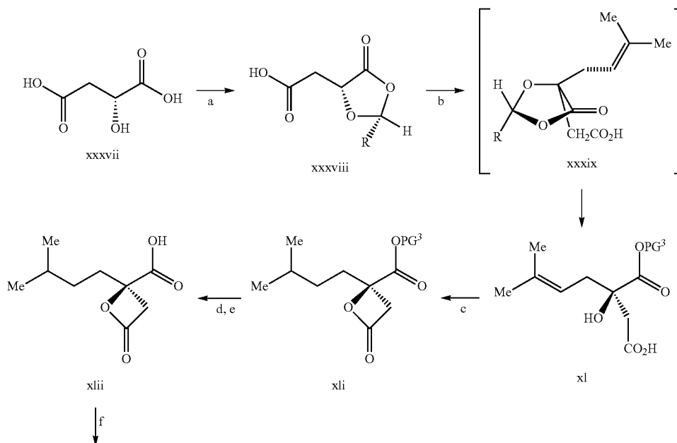
Scheme 10.
