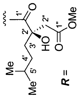
Deoxyharringtonine (2)
