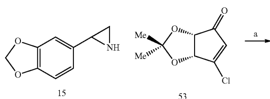
Scheme 9-1.
