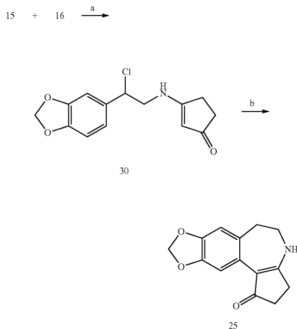
Scheme 3-1.
