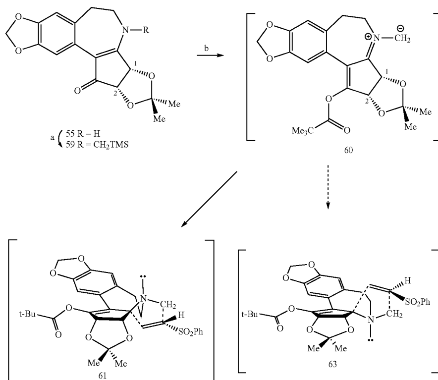
Scheme 11-1.
