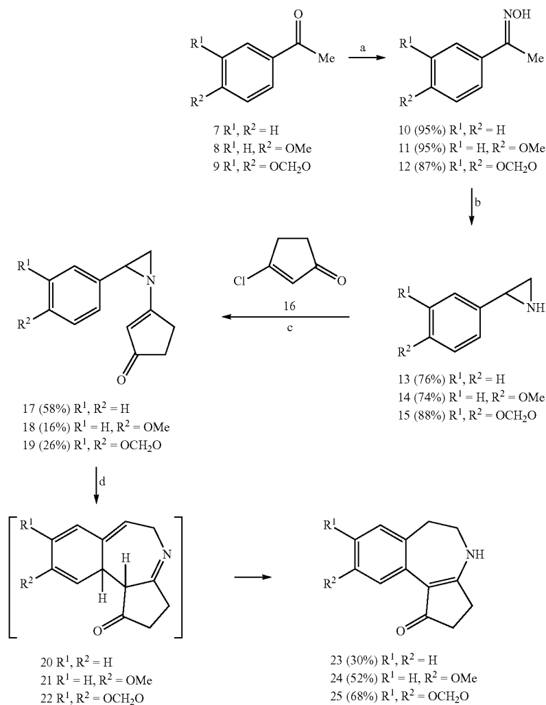
Scheme 1-1.
