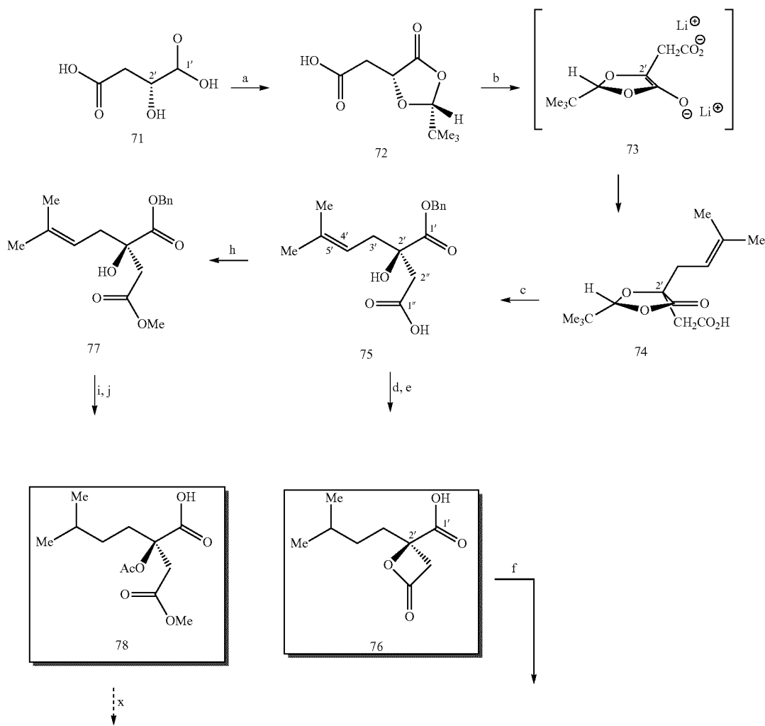
Scheme 13-1.
