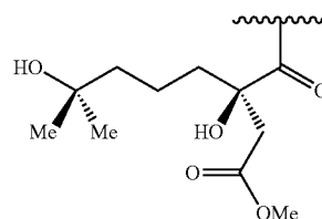
R = Homoharringtonine
