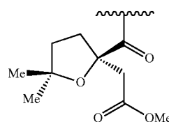
R = Anhydroharringtonine
