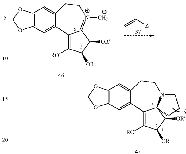
Scheme 7-1.
