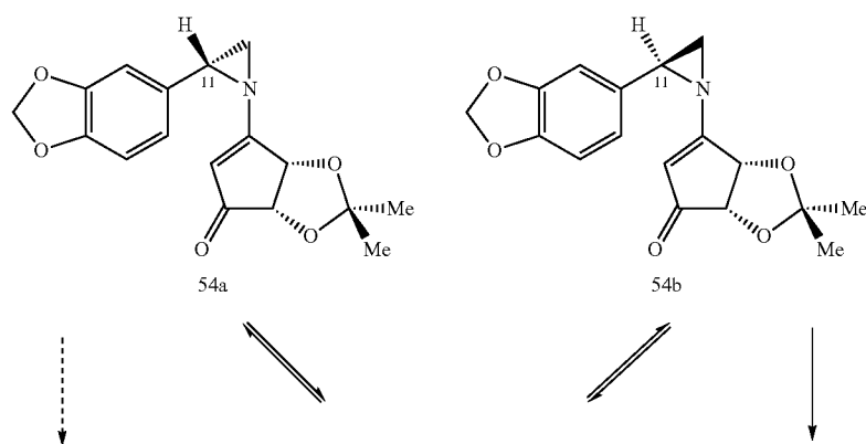
Scheme 10-1.
