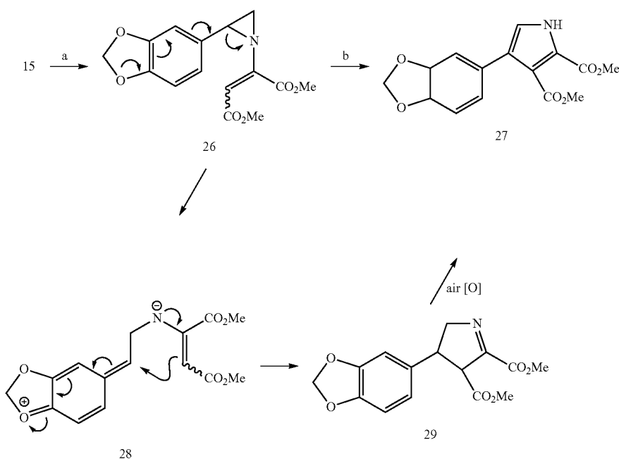
Scheme 2-1.
