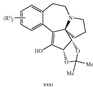
Scheme 9.
