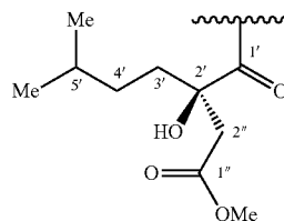
R = Deoxyharringtonine
