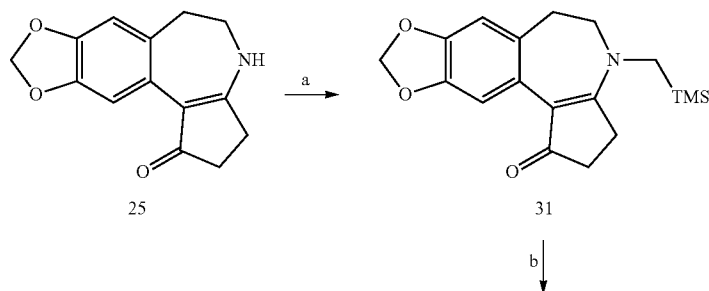
Scheme 4-1.
