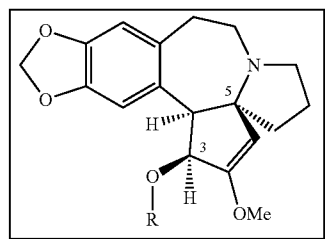
R = H Cephalofaxine
