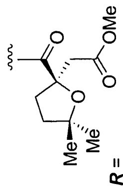
Anhydroharringtonine (5)
