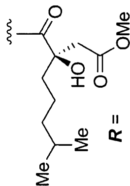
Homodeoxyharringtonine (4)
