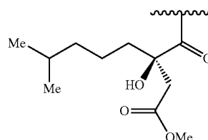
R = Homodeoxyharringtonine
