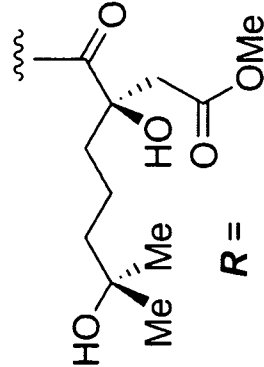
Homoharringtonine (3)
