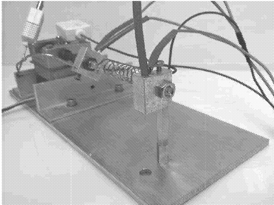
FIG. 6. MVP breadboard with 30 cm coiled tube.
