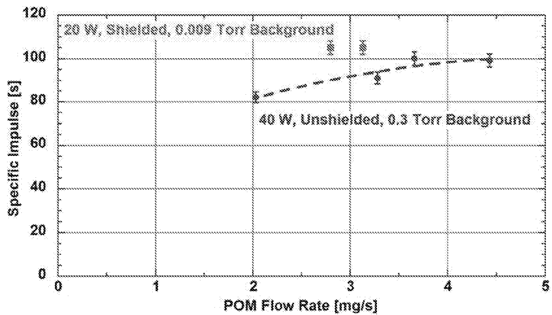
FIG. 15. Comparison between shielded and unshielded two-stage superheaters, POM propellant
