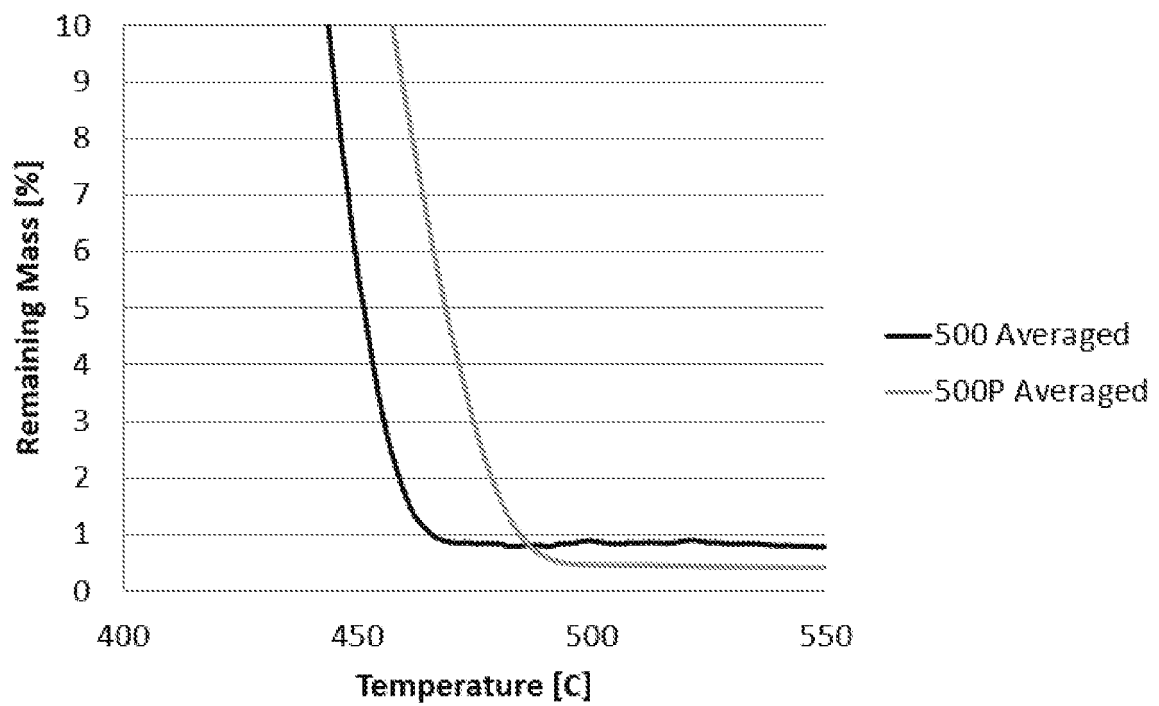
FIG. 20. TGA results for Delrin 500 and 500P
