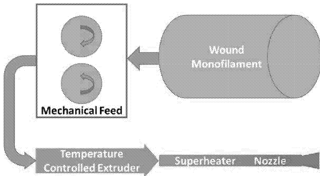
FIG. 2. MVP Block Diagram
