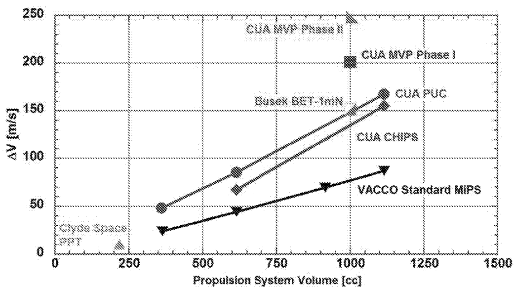
FIG. 3. \Delta V for a 4 kg satellite vs. propulsion system volume for various electric propulsion systems
