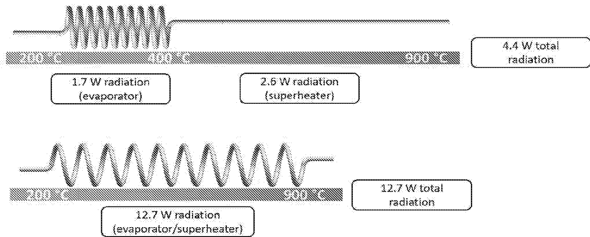
FIG. 11. Radiation modeling of superheater variants
