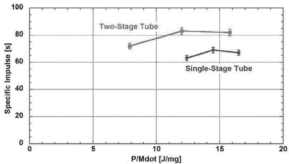
FIG. 13. Superheater tube geometry performance comparison, POM propellant
