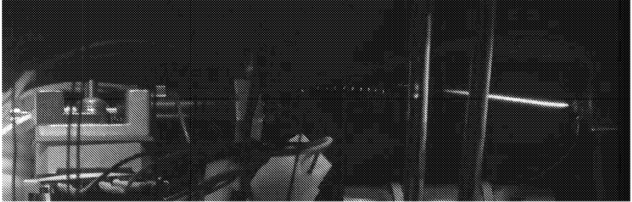
FIG. 12. Two-stage superheater operation with flowing propellant (flow is left to right).
