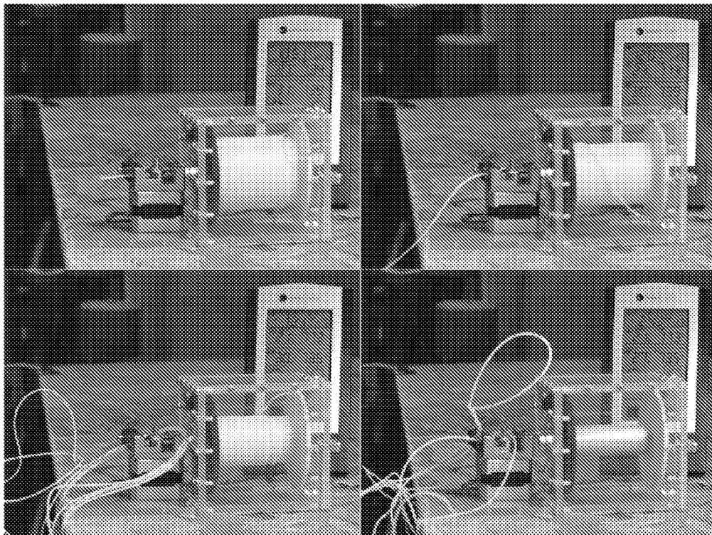
FIG. 16. Propellant storage and feed methodology. Fiber is fed around spool rim into the core.
