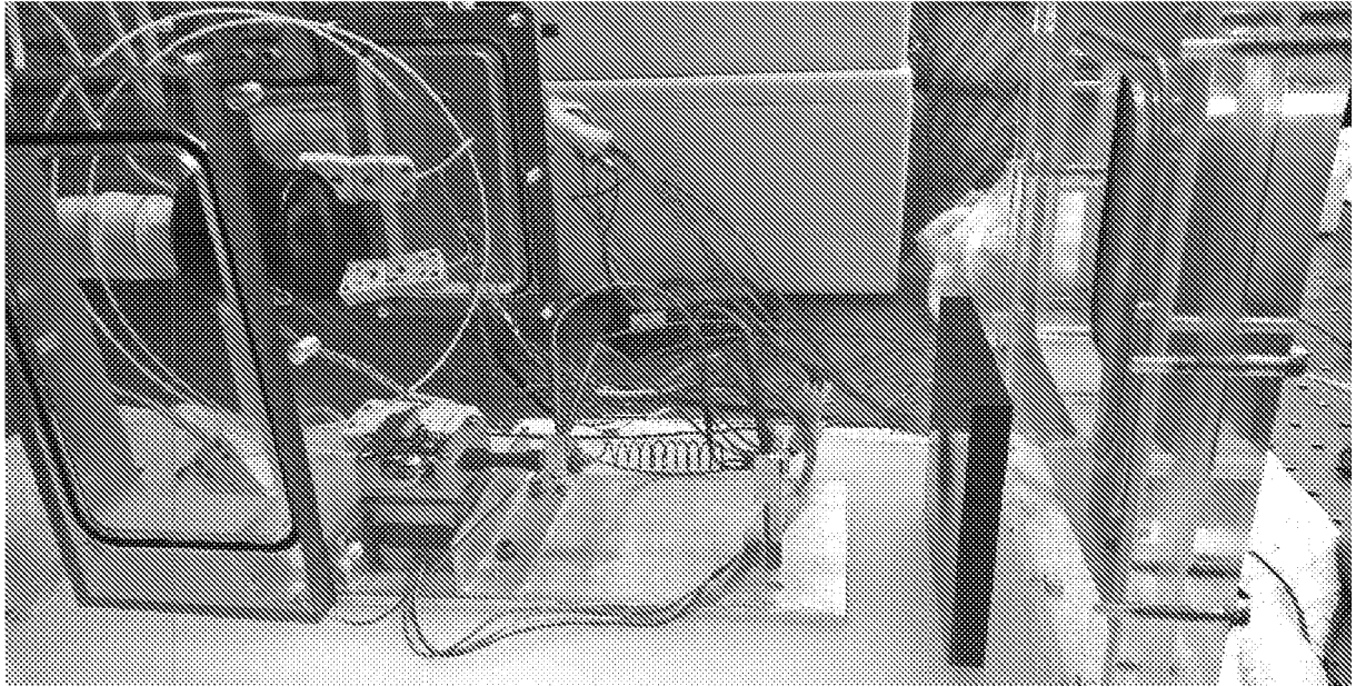
FIG. 8. MVP breadboard in clear acrylic vacuum tank
