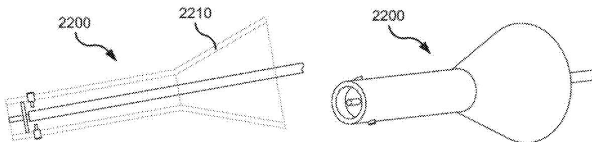
HE11 Mode Launcher
