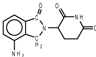
1-oxo-2-(2,6-dioxopiperidin-3-yl)-4-aminoisoindoline;
