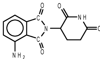
1,3-dioxo-2-(2,6-dioxopiperidin-3-yl)-4-aminoisoindoline; and
