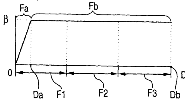
FIG. 4 (B) THROTILE POSITION MAP AFTER WARNING-UP
