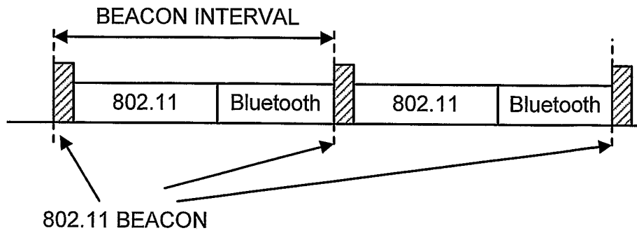
FIG. 3 (PRIOR ART)
